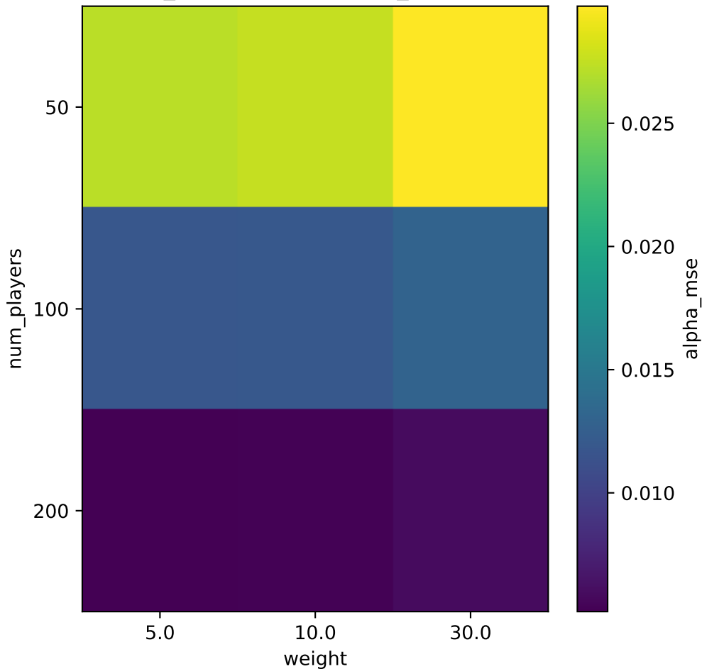
alpha_mse (avg over num_timesteps)
