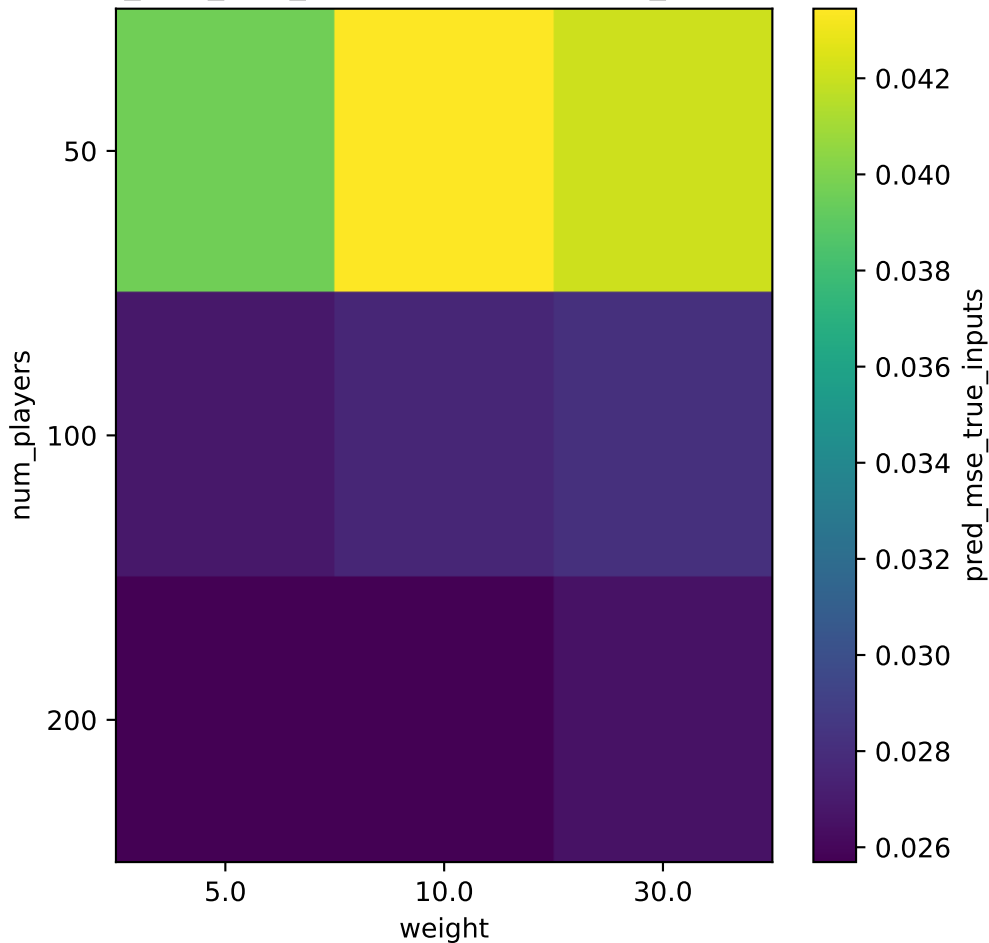
pred_mse_true_inputs (avg over num_timesteps)
