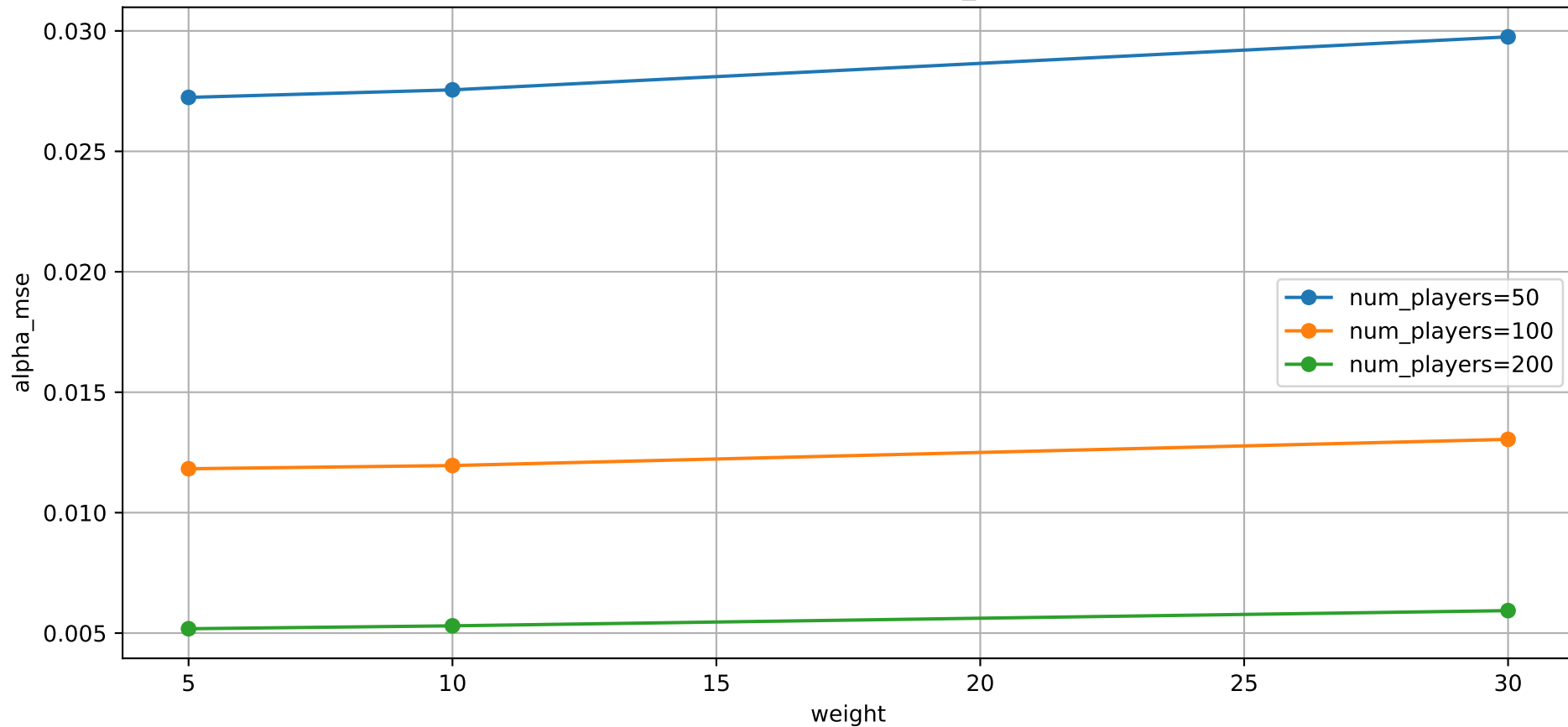
Marginal over T: alpha_mse
