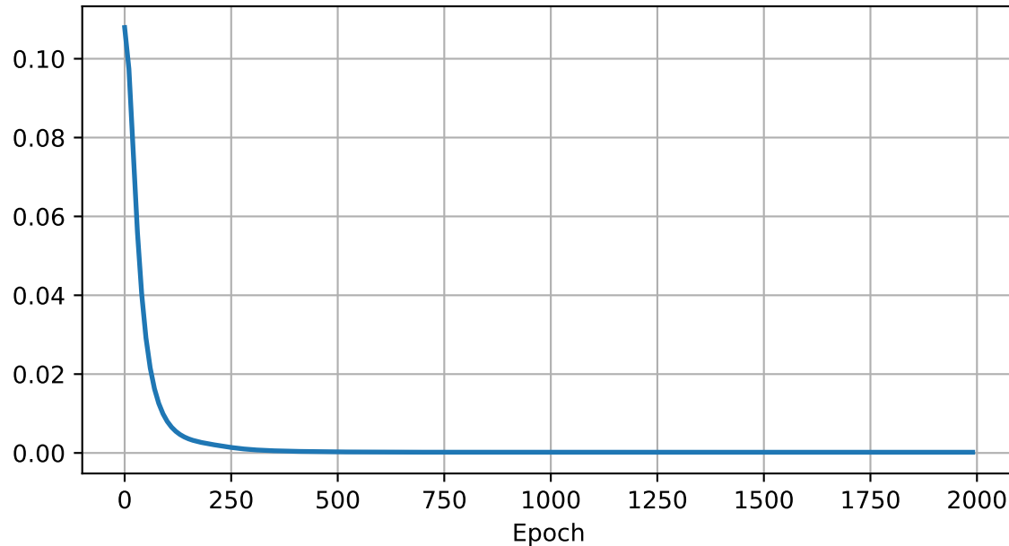
Transition BTL-Probability MSE
