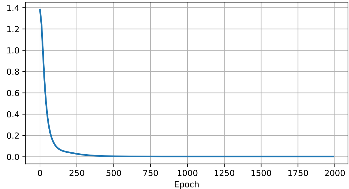
Transition Map MSE vs True Phi
