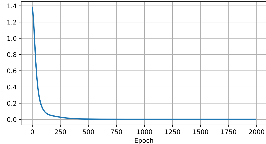
Transition State MSE
