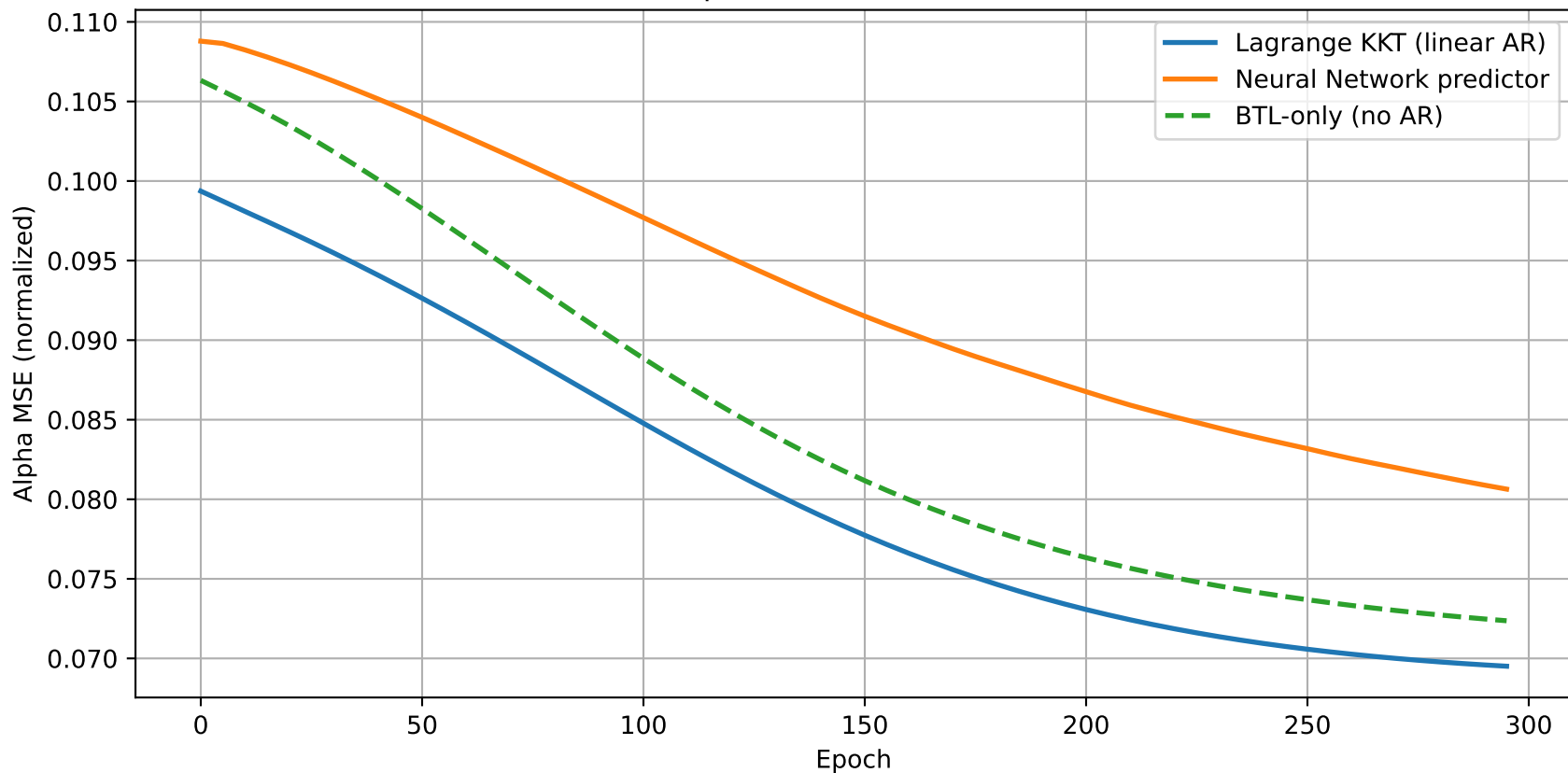
Skill recovery: Lagrange KKT vs NN vs BTL-only ( n=20 , p=3 , T=30 , \lambda=30.0 , \sigma=0.1 )
