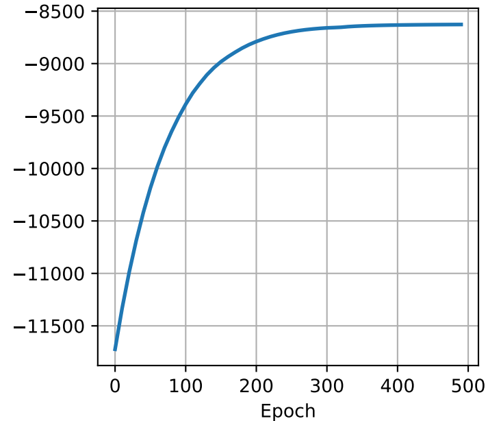
BTL Likelihood
