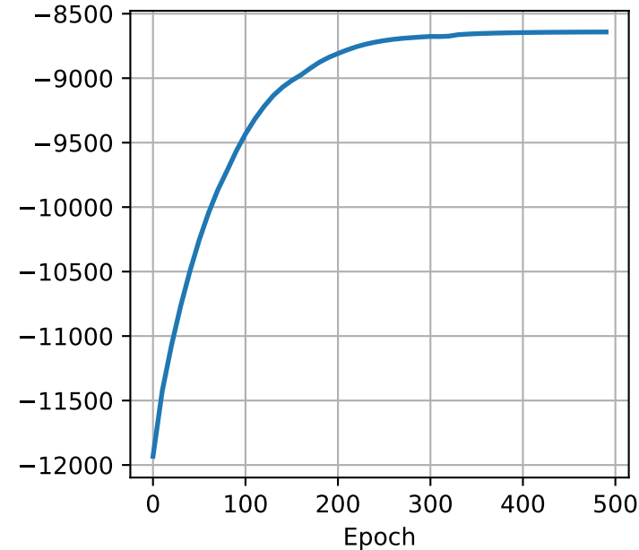
Total Likelihood
