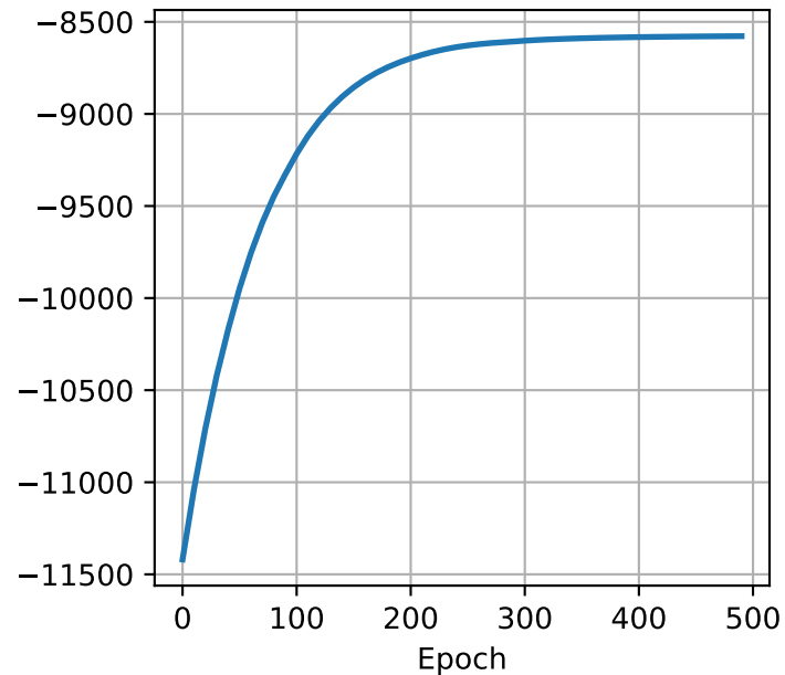
BTL Likelihood
