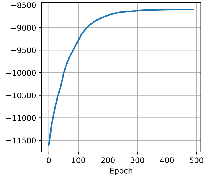
Total Likelihood
