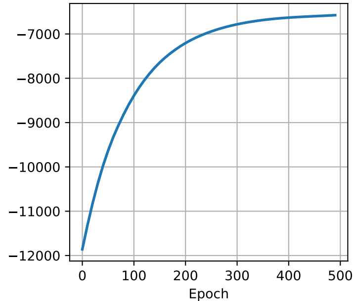
BTL Likelihood
