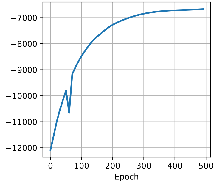
Total Likelihood
