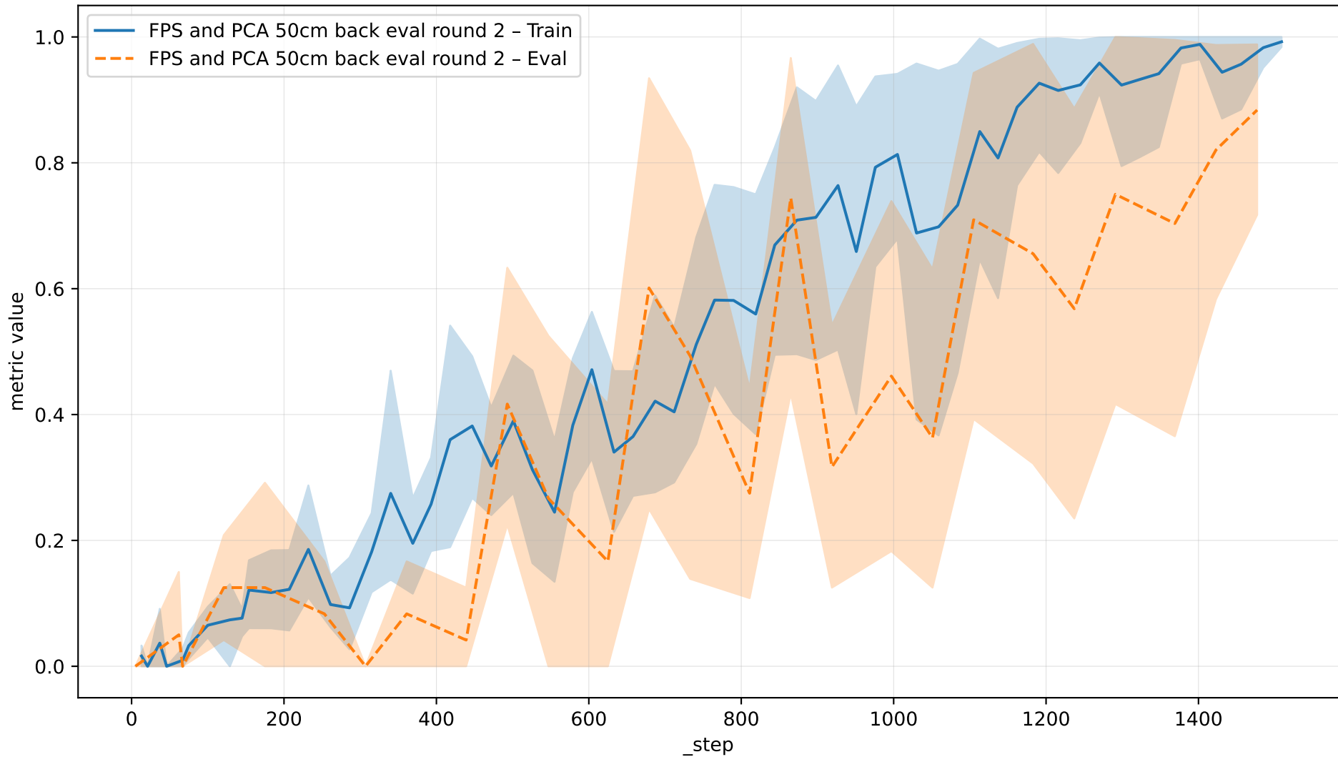
WandB curves with 95 % bootstrap CI
