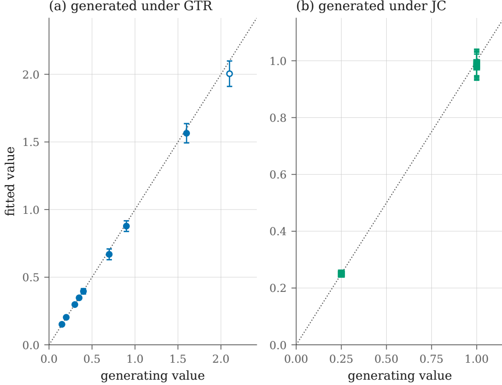
Figure 8: Fitting the general time-reversible model: five free exchangeabilities (the sixth is pinned at 1) and four stationary frequencies, alongside the branch lengths, by the same model-agnostic optimizer used for the Potts and hidden Markov instances. Bars are 95 percent Wald intervals from the observed information; the dotted line is y = x ; markers are open where an interval misses. Topology: the 2-child-root fixture, seed 20260904, 20000 sites. (a) Data simulated under an asymmetric truth, 8 of 9 intervals covering. (b) Data simulated under Jukes-Cantor, where every exchangeability is 1 and every frequency 1/4 : 9 of 9 covering. The second panel is the half that is easy to forget. A model flexible enough to fit panel (a) is only useful if it also declines to invent structure that is not there, and Jukes-Cantor is exactly the point of the parameter space where the general model could most easily do so. Coverage on a single dataset is a draw and not a rate: the nominal 0.95 is checked over independent replicates by the release-gated regression suite.
