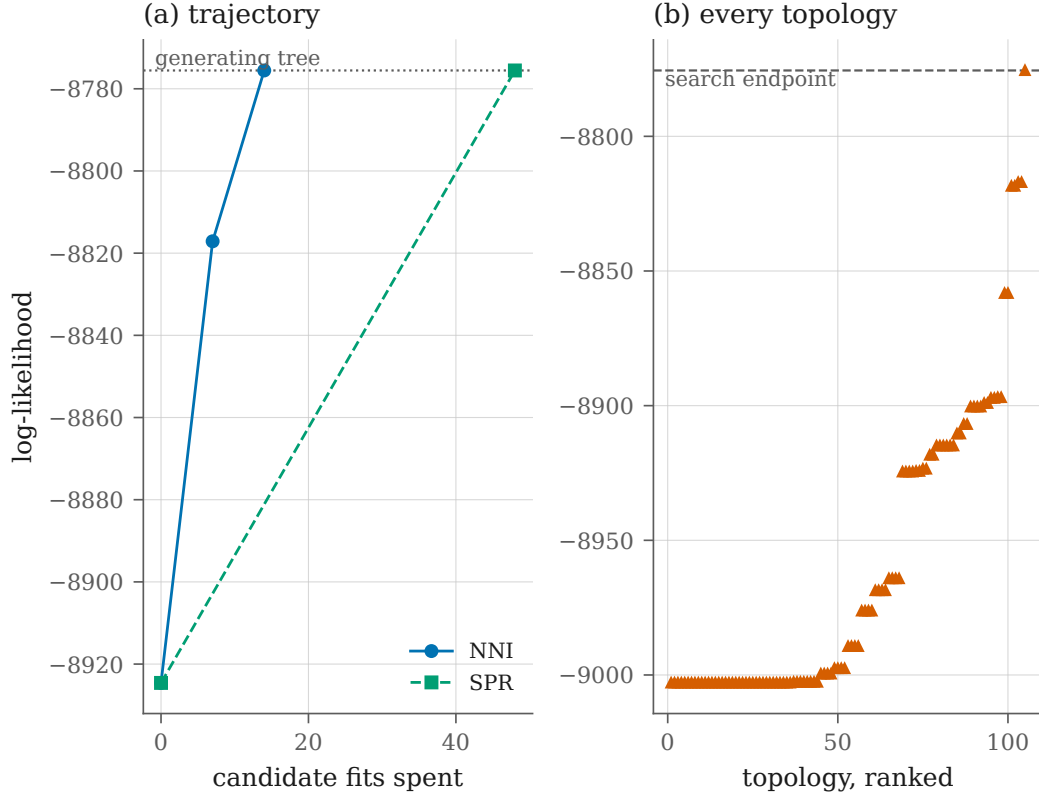
Figure 9: Hill climbing over tree topologies, scoring every candidate with the same model-agnostic optimizer used for the Potts and hidden Markov instances. Fixture: 4-state Jukes-Cantor, 1500 sites, seed 20260905. (a) Log-likelihood against candidate fits spent, from a randomly drawn starting topology; the dotted line is the generating tree’s own score. (b) All 105 unrooted topologies on this leaf set, scored and ranked, with the search’s endpoint dashed. Below 8 taxa this enumeration is affordable, which is what makes the phrase found the best tree a checkable claim rather than an assertion. The optimum leads the runner-up by 41.6 log units here, so this problem does not yet separate the two move sets: both reach it, NNI in fewer fits.
