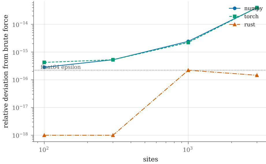
Figure 4: Every pruning backend against the oracle that owes it nothing. Brute-force marginalization sums over all ancestral assignments, so it shares no code with the recursion it checks, and its cost is what keeps the fixture small. Fixture: 4-state Jukes-Cantor on the 3-child-root tree, seed 20260902. The deviation is relative because the log-likelihood is a sum over sites: an absolute bound fixed at one site count does not transfer to another, which is why the x-axis spans a factor of 30. Worst deviation across every backend and size: 3.99e-14, against a float64 epsilon of 2.22e-16.
