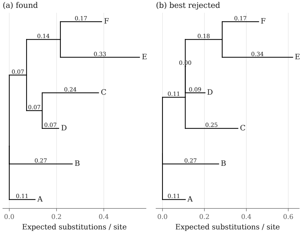
Figure 10: The topology hill climbing selected, beside the highest-scoring one it rejected, each with its own branch lengths fitted. Fixture: 4-state Jukes-Cantor over 1500 sites, seed 20260905. (a) scores -8775.5 and is the generating topology; (b) scores -8817.1, a difference of 41.6 log units. They differ by one split: C D are a group in one and not in the other. On this fixture the search recovers the generating tree, so a drawing of found against true would show the same tree twice; the runner-up is what the likelihood actually had to discriminate against. Note its shortest internal branch, fitted at 0.000: a wrong grouping is generally only supportable by collapsing the edge that would create it.
