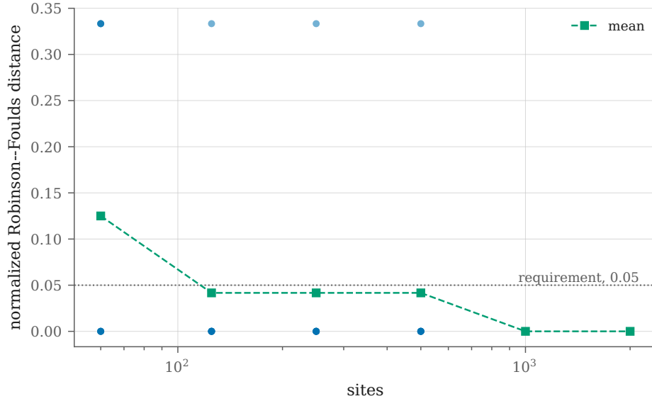
Figure 11: How much alignment the search needs to recover the tree that generated it. Each marker is one independent alignment drawn from the 4-state Jukes-Cantor fixture (seed 20260905, 8 replicates per size), inferred by NNI hill climbing and scored against the generating topology by normalized Robinson-Foulds distance – 0 for the same tree, 1 for no internal split in common. The dotted line is the accuracy requirement this project set itself, 0.05. It is met from 125 sites upward: 8 of 8 replicates recover the topology exactly at 2000 sites, against 5 of 8 at 60. The distance is normalized by internal splits, so the bound means the same thing at any taxon count.
