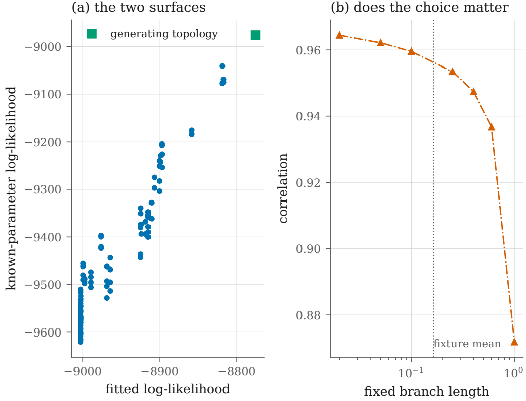
Figure 12: The reward an agent can afford, against the one it stands in for. Every one of the 105 unrooted topologies on this leaf set, scored twice: at fixed known parameters, and at parameters maximized per topology by the same optimizer the Potts and hidden Markov instances use. Fixture: 4-state Jukes-Cantor, 1500 sites, seed 20260905; the fixed branch length is the generating tree’s mean, 0.1644. (a) The two surfaces, correlation 0.9568; both score the generating topology highest, so the cheap reward and the expensive one agree on the answer while disagreeing in detail. The correlation is linear rather than rank-based because the fitted surface does not totally order topologies: several of its optima agree to within the optimizer’s own convergence, so their relative order is not a property of the model. (b) The cheap surface has one free parameter, and the conclusion does not rest on it: across a 50-fold range of fixed branch length the two surfaces pick the same best topology in 7 of 7 cases, with the correlation never falling below 0.8719. The substitution is what makes training affordable at all: the fitted reward runs a full optimization per candidate, the known one a single pruning pass.
