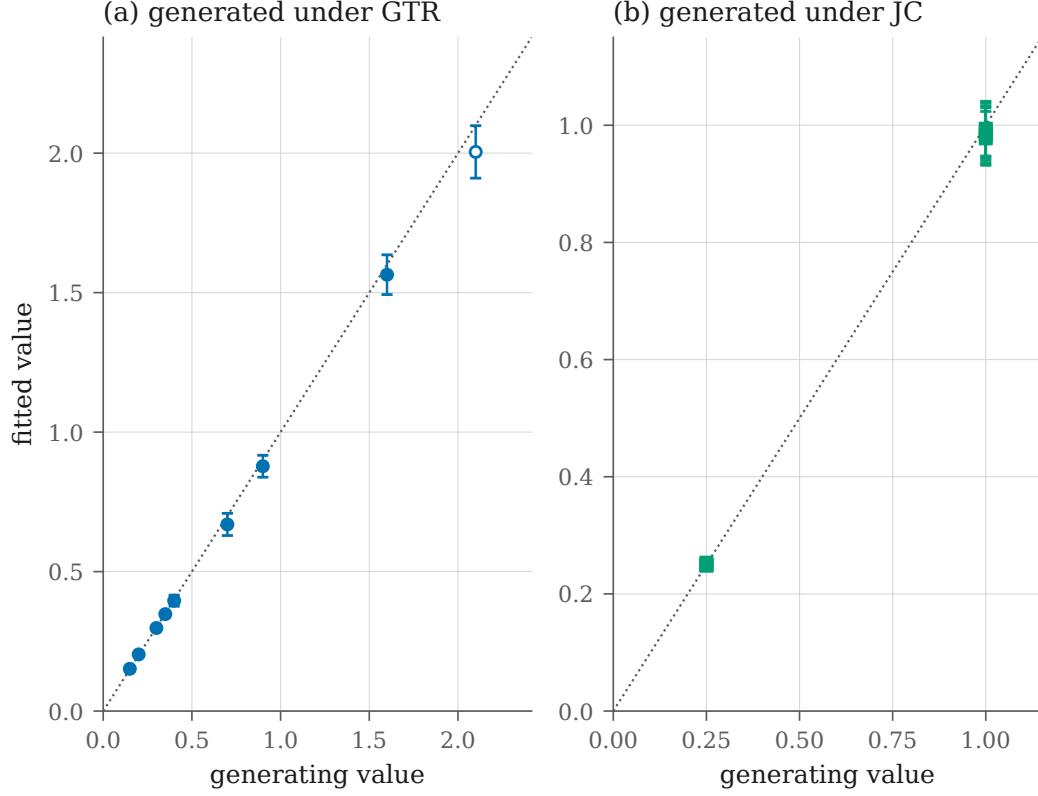
Figure 9: Fitting the general time-reversible model: five free exchangeabilities (the sixth is pinned at 1) and four stationary frequencies, alongside the branch lengths, by the same model-agnostic optimizer used for the Potts and hidden Markov instances. Bars are 95 percent Wald intervals from the observed information; the dotted line is y = x ; markers are open where an interval misses. Topology: the 2-child-root fixture, seed 20260904, 20000 sites. (a) Data simulated under an asymmetric truth, 8 of 9 intervals covering. (b) Data simulated under Jukes-Cantor, where every exchangeability is 1 and every frequency 1/4 : 9 of 9 covering. The second panel is the half that is easy to forget. A model flexible enough to fit panel (a) is only useful if it also declines to invent structure that is not there, and Jukes-Cantor is exactly the point of the parameter space where the general model could most easily do so. Coverage on a single dataset is a draw and not a rate: the nominal 0.95 is checked over independent replicates by the release-gated regression suite.
