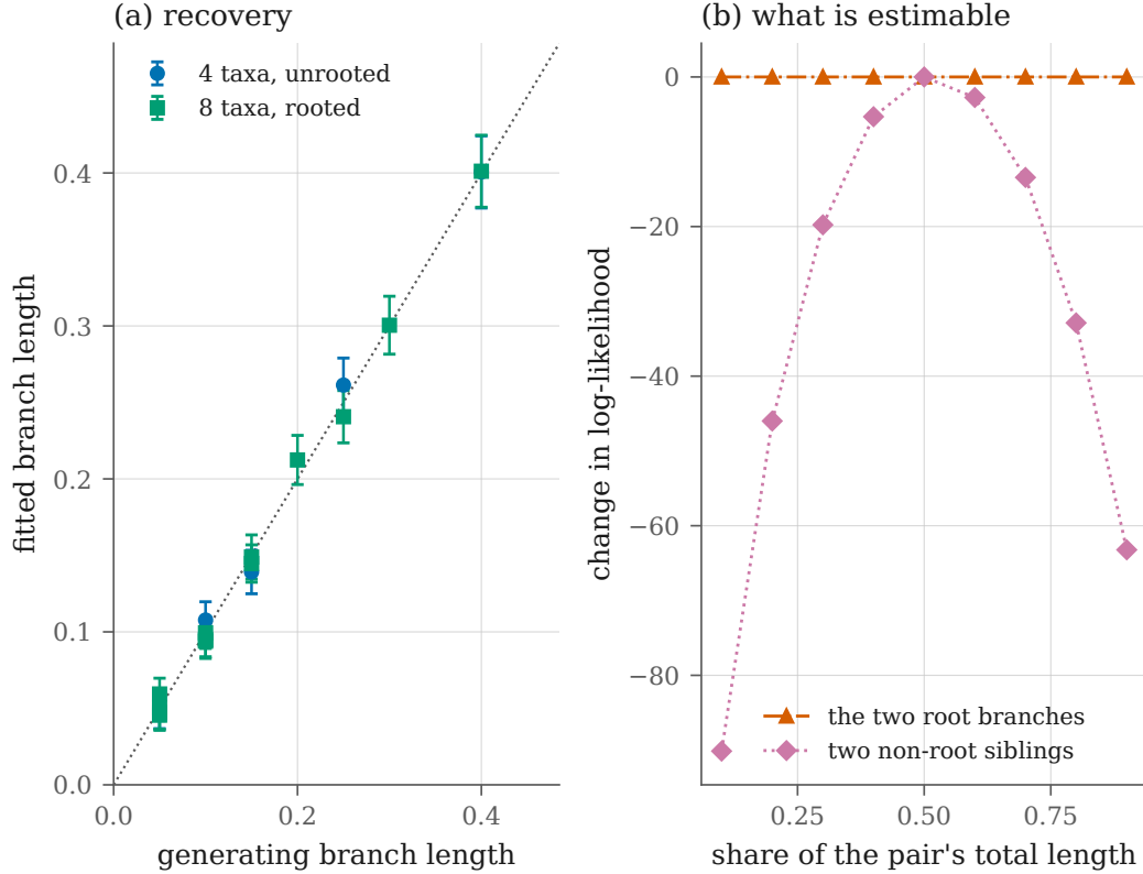
Figure 8: Branch-length fitting by autodiff, using the same model-agnostic optimizer as the Potts and hidden Markov instances. (a) Every estimable branch length against the value that generated the alignment, with 95 percent Wald intervals from the observed information; markers are open where an interval misses. Fixtures: 3-child root, seed 20260903, and 2-child root, seed 20260904, both scored at 5000 sites. (b) Why some branch lengths are not estimable at all. Moving mass between the two branches below a rooted binary tree's root, at fixed sum, changes the log-likelihood not at all: the log-likelihood is bit-identical across a 9 to 1 range. The same move between two non-root siblings changes it by up to 90.1. This is the pulley principle: under a reversible model the likelihood does not depend on where the root sits along the branch it subdivides. Only the pair's sum is estimable, so the objective fits it as one parameter; fitting both would leave the observed information singular and every interval in panel (a) undefined.
