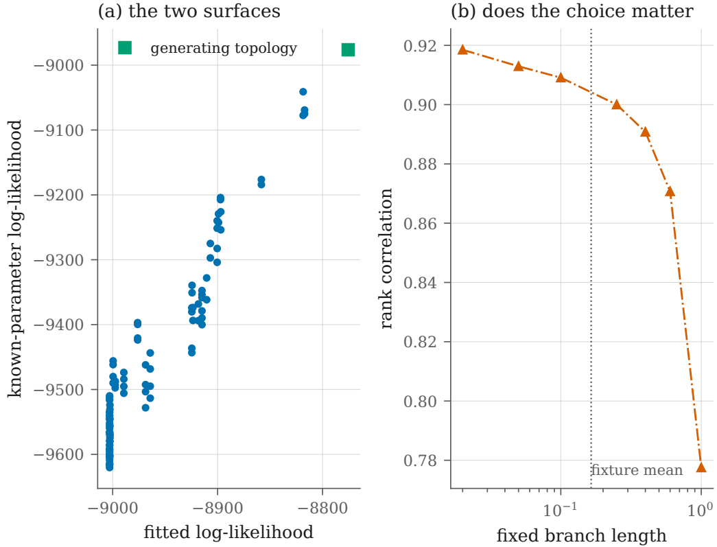
Figure 10: The reward an agent can afford, against the one it stands in for. Every one of the 105 unrooted topologies on this leaf set, scored twice: at fixed known parameters, and at parameters maximized per topology by the same optimizer the Potts and hidden Markov instances use. Fixture: 4-state Jukes-Cantor, 1500 sites, seed 20260905; the fixed branch length is the generating tree’s mean, 0.1644. (a) The two surfaces, rank correlation 0.9045; both rank the generating topology first, so the cheap reward and the expensive one agree on the answer while disagreeing in detail. (b) The cheap surface has one free parameter, and the conclusion does not rest on it: across a 50-fold range of fixed branch length the two surfaces pick the same best topology in 7 of 7 cases, with the rank correlation never falling below 0.7775. The substitution is what makes training affordable at all: the fitted reward runs a full optimization per candidate, the known one a single pruning pass.
