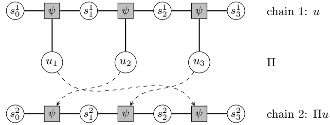
Figure 18: A turbo code as a factor graph: two trellis chains sharing the message bits through a permutation. Each \psi is one trellis factor of Equation 26, carrying both the transition the register allows and the channel's score for the two bits that transition transmits; each s_t^c is a register state. The message bit u_i is read by the first chain at position i and by the second at position \Pi^{-1}(i) , so every u_i has degree two and the graph has one cycle per pair of message bits the permutation reorders — which is why Equation 2 on it is the Bethe approximation and why the serial schedule of Algorithm 17 is a choice rather than a derivation. Three message bits and a memory-1 register are drawn; the instances this repository carries are K = 12, 256 and 1,024 with the memory-2 (7, 5) register. A sketch of the structure and not a rendering of any instance.
