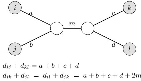
Figure 21: The four-point condition, Equation 50, on the quartet resolved as ij \mid kl . Each of the two larger pairing sums crosses the interior edge twice, so the two are equal and each exceeds the smallest by 2m ; the smallest sum names the resolution. A quartet with m = 0 is unresolved and all three sums agree, which is why an estimated matrix recovers a quartet only when its error is below the interior length — Atteson’s radius, in one quartet.
