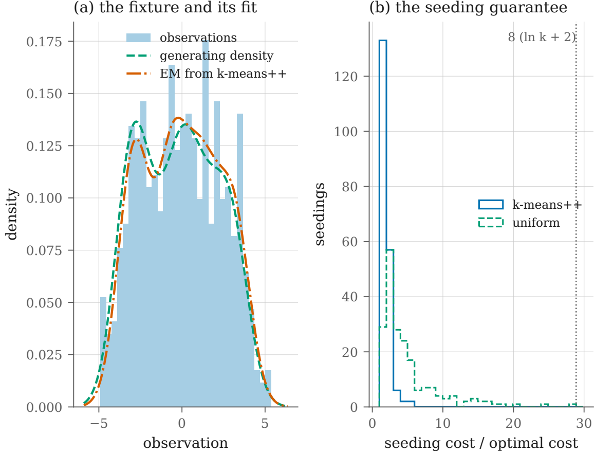
Figure 4: A Gaussian mixture of 5 components with means -3, -1.5, 0, 1.5, 3, unit scales and weights 0.3, 0.1, 0.25, 0.15, 0.2: 500 observations at seed 20260908. (a) The observations, the generating density, and the density expectation-maximization reaches from one k-means++ start at the 500-iteration cap, still moving, at log-likelihood -1122.3. (b) The k-means cost of a seeding divided by the exact optimal cost from the one-dimensional dynamic programme, over 200 independent seedings of the same observations each way: k-means++ averages 1.90 (worst 5.61) and uniform seeding 4.95 (worst 28.68), against the published bound of 28.88 on the k-means++ expectation. The bound is a statement about the mean, and the mean is what is held to it.
