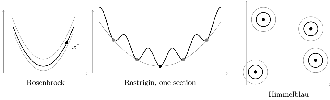
Figure 1: The three surfaces, schematically. Rosenbrock is a single curved valley whose difficulty is conditioning alone, and its minimizer is the marked point of Equation 8. Rastrigin, drawn as one one-dimensional section, is a quadratic bowl under a cosine ripple: the black point is the global minimum of Equation 9 and every grey point a local minimum satisfying the same first-order condition, of which there are about 10^d in d dimensions. Himmelblau has four minima of equal value, Equation 10, so “the” optimum is not a well-formed question and a method that always returns one basin is reading its start. A sketch of the shape of each surface, not a rendering of any of them; the rendered surfaces are Figure 2.
