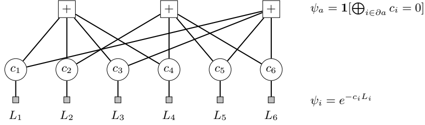
Figure 16: A Tanner graph: bits c_i \in \{0, 1\} as circles, the parity factors of a row of \mathbf{H} as squares, and the channel factor of Equation 25 as a shaded square carrying the log-likelihood ratio L_i at each bit. The drawn graph is six bits and three checks of degree four; the ensemble this repository carries is regular (3, 6) , so every bit sits on three parity factors and every parity factor on six bits. The graph has cycles — a random draw of the ensemble does not avoid short ones — so Equation 7 on it is the Bethe approximation and Equation 83 is that approximation in the log domain. A sketch of the structure and not a rendering of any instance.
