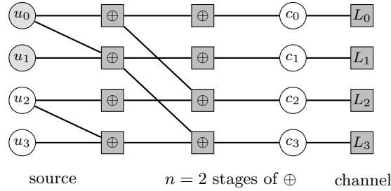
Figure 20: The transform of Equation 40 at N = 4 as a factor graph. Each \oplus is one application of the kernel: a parity factor over the pair it joins. Shaded source variables are frozen to zero and carry no message, and which they are is what Equation 42 chooses. Successive cancellation is a schedule on this graph and not a separate algorithm — it decides u_0 , then u_1 given that decision, and so on, each pass exact given the ones before it.
