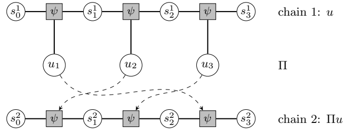
Figure 18: A turbo code as a factor graph: two trellis chains sharing the message bits through a permutation. Each \psi is one trellis factor of Equation 39, carrying both the transition the register allows and the channel's score for the two bits that transition transmits; each s_t^c is a register state. The message bit u_i is read by the first chain at position i and by the second at position \Pi^{-1}(i) , so every u_i has degree two and the graph has one cycle per pair of message bits the permutation reorders — which is why Equation 7 on it is the Bethe approximation and why the serial schedule of Algorithm 18 is a choice rather than a derivation. Three message bits and a memory-1 register are drawn; the instances this repository carries are K = 12, 256 and 1,024 with the memory-2 (7, 5) register. A sketch of the structure and not a rendering of any instance.
