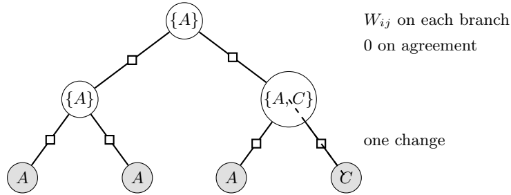
Figure 9: One site of large parsimony as the same tree factor graph in the min-plus semiring. Shaded circles are the observed characters, open circles the Fitch sets of Equation 61 carried up the tree, and squares the branch factors, whose table is 0 on agreement and W_{ij} otherwise (Equation 62). The right-hand cherry disagrees, so its parent takes the union and the site's score is one change, drawn dashed on the branch that pays it. The structure is Figure 7 with the probabilities replaced by costs and the branch lengths removed; the search over the (2n - 5)!! topologies is what makes the problem large parsimony. A sketch of the structure and not a rendering of any instance.
