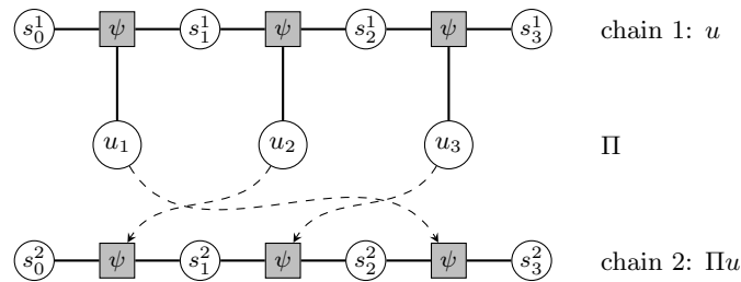
Figure 18: A turbo code as a factor graph: two trellis chains sharing the message bits through a permutation. Each \psi is one trellis factor of Equation 29, carrying both the transition the register allows and the channel's score for the two bits that transition transmits; each s_t^c is a register state. The message bit u_i is read by the first chain at position i and by the second at position \Pi^{-1}(i) , so every u_i has degree two and the graph has one cycle per pair of message bits the permutation reorders — which is why Equation 2 on it is the Bethe approximation and why the serial schedule of Algorithm 17 is a choice rather than a derivation. Three message bits and a memory-1 register are drawn; the instances this repository carries are K = 12, 256 and 1,024 with the memory-2 (7, 5) register. A sketch of the structure and not a rendering of any instance.
