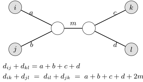
Figure 21: The four-point condition, Equation 53, on the quartet resolved as ij \mid kl . Each of the two larger pairing sums crosses the interior edge twice, so the two are equal and each exceeds the smallest by 2m ; the smallest sum names the resolution. A quartet with m = 0 is unresolved and all three sums agree, which is why an estimated matrix recovers a quartet only when its error is below the interior length — Atteson’s radius, in one quartet.
