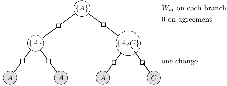
Figure 9: One site of large parsimony as the same tree factor graph in the min-plus semiring. Shaded circles are the observed characters, open circles the Fitch sets of Equation 47 carried up the tree, and squares the branch factors, whose table is 0 on agreement and W_{ij} otherwise (Equation 48). The right-hand cherry disagrees, so its parent takes the union and the site's score is one change, drawn dashed on the branch that pays it. The structure is Figure 7 with the probabilities replaced by costs and the branch lengths removed; the search over the (2n - 5)!! topologies is what makes the problem large parsimony. A sketch of the structure and not a rendering of any instance.
