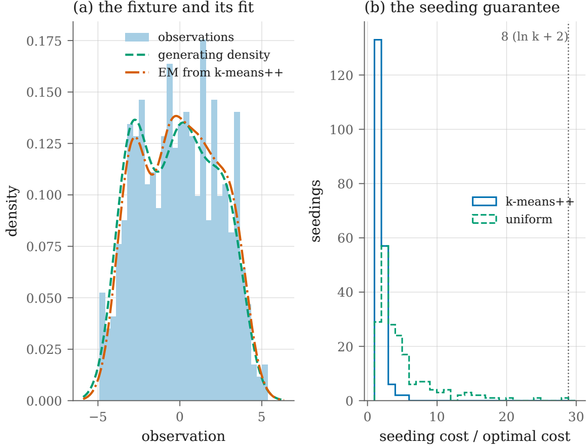
Figure 6: A Gaussian mixture of 5 components with means -3, -1.5, 0, 1.5, 3 , unit scales and weights 0.3, 0.1, 0.25, 0.15, 0.2 : 500 observations at seed 20260908. (a) The observations, the generating density, and the density expectation-maximization reaches from one k-means++ start at the 500-iteration cap, still moving, at log-likelihood -1122.3 . (b) The k-means cost of a seeding divided by the exact optimal cost from the one-dimensional dynamic programme, over 200 independent seedings of the same observations each way: k-means++ averages 1.90 (worst 5.61) and uniform seeding 4.95 (worst 28.68), against the published bound of 28.88 on the k-means++ expectation. The bound is a statement about the mean, and the mean is what is held to it.
