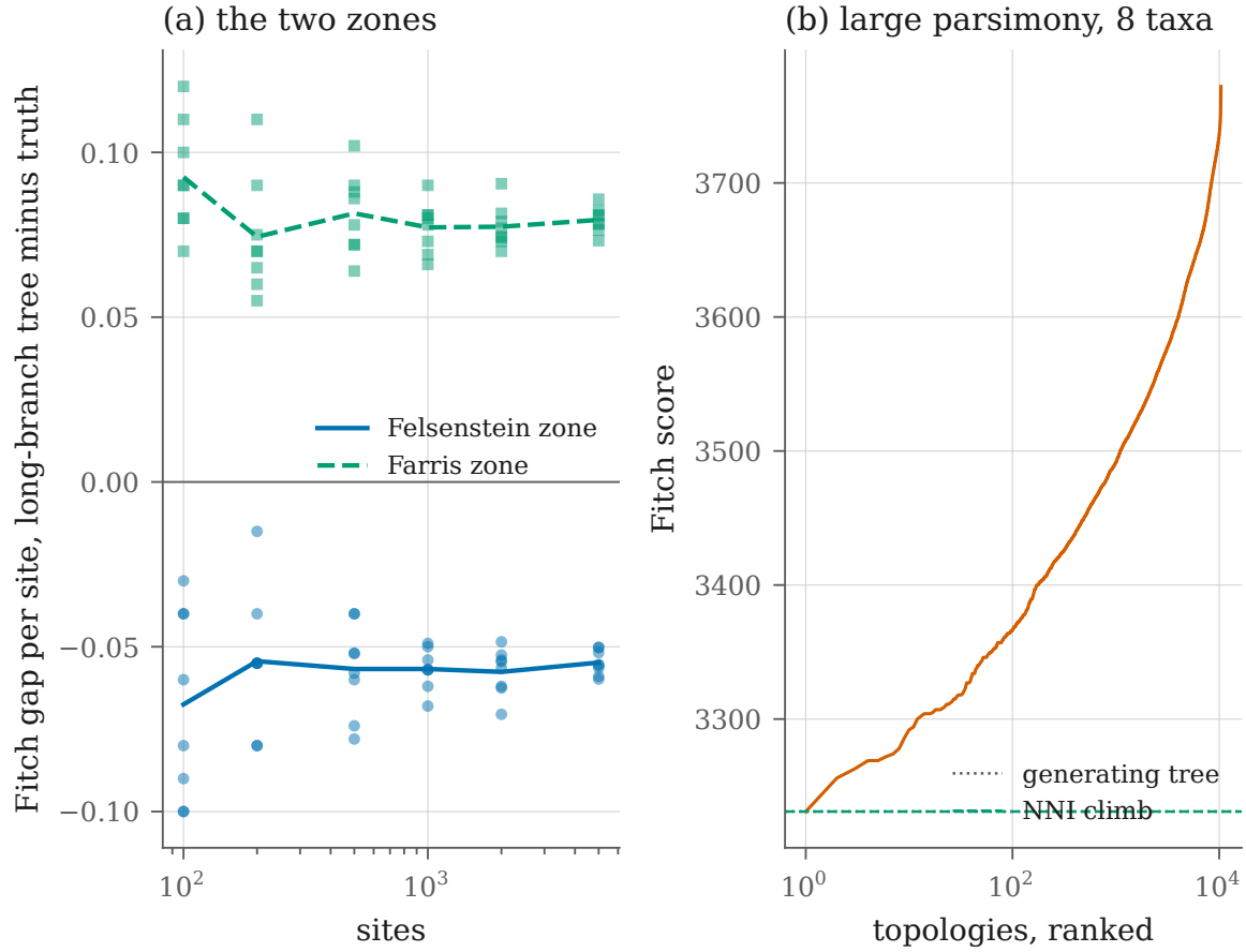
Figure 4: Parsimony in the two zones, and large parsimony on the eight-taxon fixture. (a) Four taxa, pendant branches 0.75 and 0.02 expected substitutions per site with internal branches 0.02, 4-state Jukes-Cantor, seed 20260904, 8 independent alignments at each of 6 site counts from 100 to 5000. Each marker is the Fitch score of the tree grouping the two long branches minus the generating tree's, per site; the line is the mean. In the Felsenstein zone the long branches are not a cherry and the mean gap is -0.068 at 100 sites and -0.055 at 5000: negative, so the criterion prefers the wrong tree, and not closing, which is statistical inconsistency. In the Farris zone the same branches are a cherry and the gap is 0.092 and 0.080. (b) Every one of the 10_395 unrooted topologies on the 8-taxon fixture, scored at 2000 sites (seed 20260904) and ranked; the generating tree scores 3231 and is the minimum. A nearest-neighbour-interchange climb from a random start reaches 3231 after scoring 26 candidates of a 400 budget, the generating tree; the enumeration is the oracle that says so.
