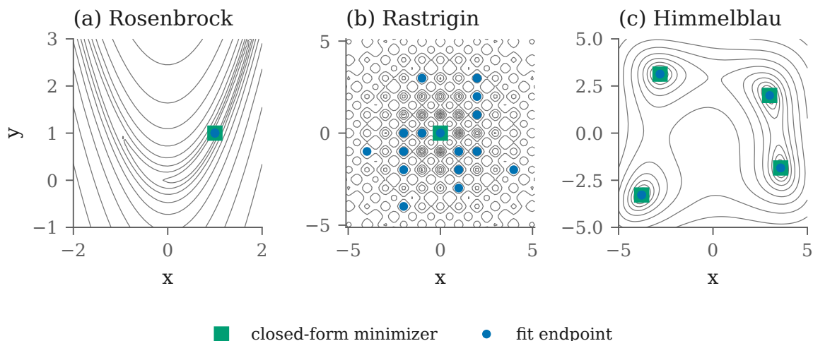
Figure 7: The three continuous test functions in two dimensions, with the minimizers known in closed form and the endpoints of L-BFGS fits from Gaussian random restarts around each function’s own start, the origin for Rastrigin (seed 20260908). (a) Rosenbrock, 4 restarts at scale 1: 4 of 4 reach the minimizer (1, 1). (b) Rastrigin, 16 restarts at scale 2: 1 of 16 reach the global minimum at the origin, every fit stopping at the local minimum of the cell it started in, so a single fit of this surface reports convergence and not optimality. (c) Himmelblau, 8 restarts at scale 3: 8 of 8 reach one of the four equal minima, which one depending on the basin the start fell in. Contours are drawn in \log(1 + \text{value}) .
