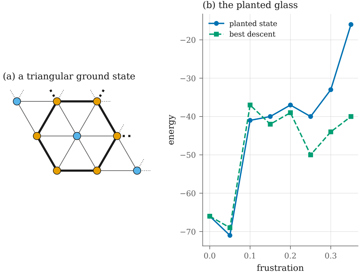
Figure 5: Two frustrated instances with an answer from outside. (a) The 3x3 periodic triangular Ising antiferromagnet, coupling -1, 27 bonds (dotted: bonds wrapping the torus), with one of its enumerated ground states coloured by spin. Heavy bonds join agreeing spins: 9 of 27, one in three, which the double count over triangles fixes as the minimum at every size, so the ground-state energy is 9 exactly. (b) A planted Viana-Bray spin glass on 60 sites at mean degree 4, couplings of magnitude 1, one instance per frustration from seed 20260908: the energy of the planted state against the lowest energy reached by 20 single-site descents from random starts. Descent lands on the planted energy at 3 of 8 frustrations and goes below it at 5, where the planted state is an upper bound on the ground state and not the ground state.
