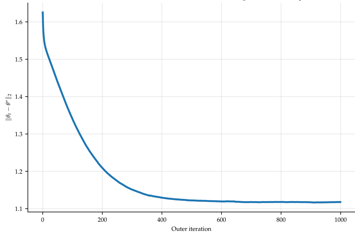
Reward L2 vs iteration — demo_betas_1.000_1.000_1.000_stage_demos — noeps — lam=0
