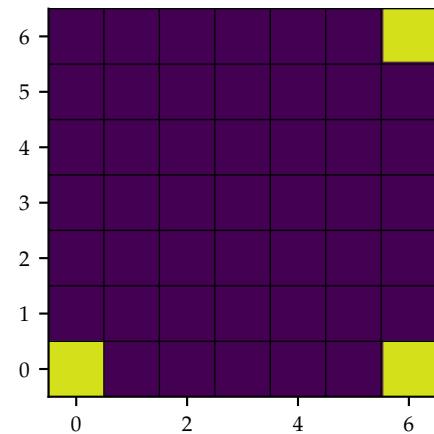
True reward
