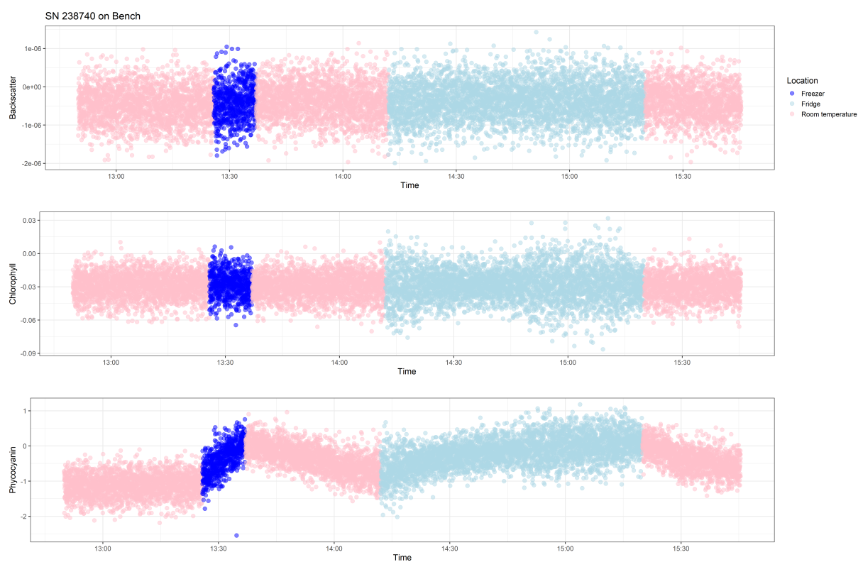
Figure 21: Serial 238740. Room temperature (20 °C), fridge (6 °C) and freezer (-18 °C). Test performed and visualized by Adele Maciute, Oceanographic Technician at Voice of the Ocean Foundation.
