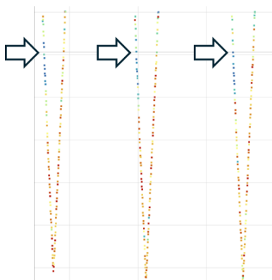
Figure 1: A lag between up- and downcast phycocyanin data was discovered at sea in August 2025.
