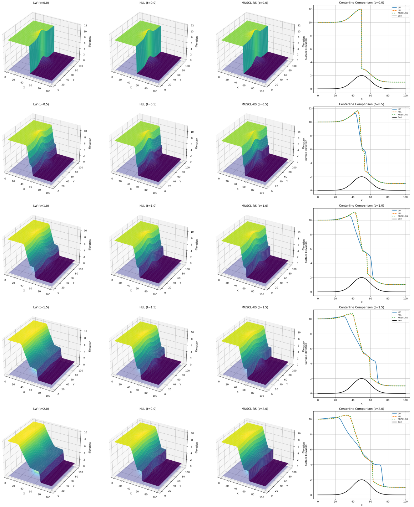
Figure 1: Comparison of the LW, HLL, and MUSCL–Rusanov schemes for the step dam-break problem at different time instances.
