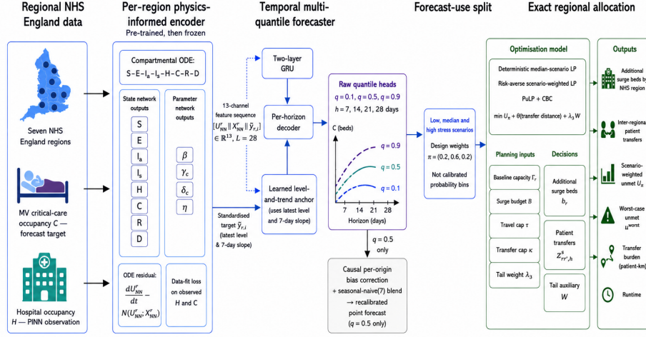
Fig. 1. Forecast-to-allocation pipeline. Frozen PINN features feed raw multi-quantile forecasts; the low, median and high heads supply the LP unchanged, whereas recalibration is restricted to point evaluation.
