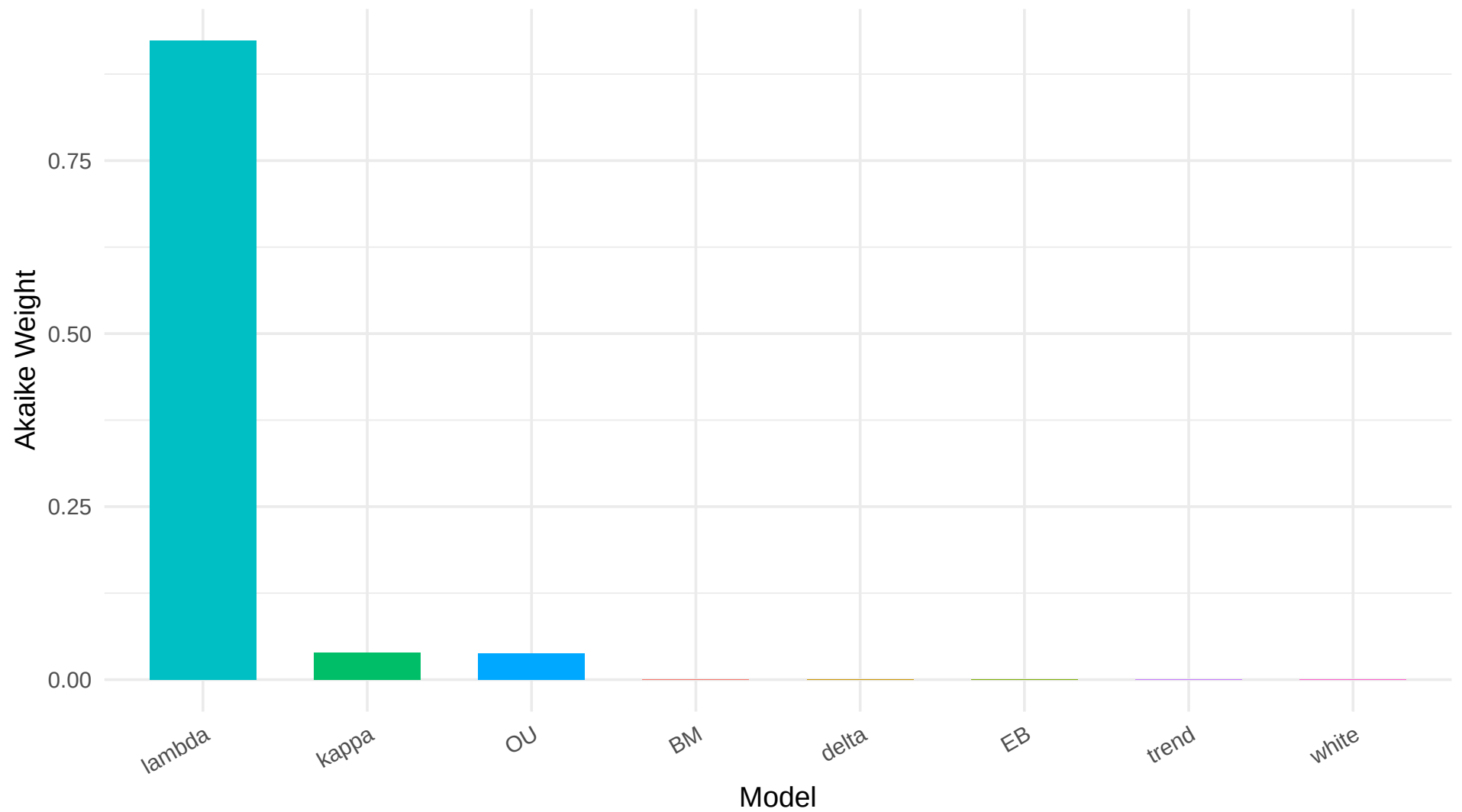
Expanded model comparison on PhyloPC1 (8 models)
