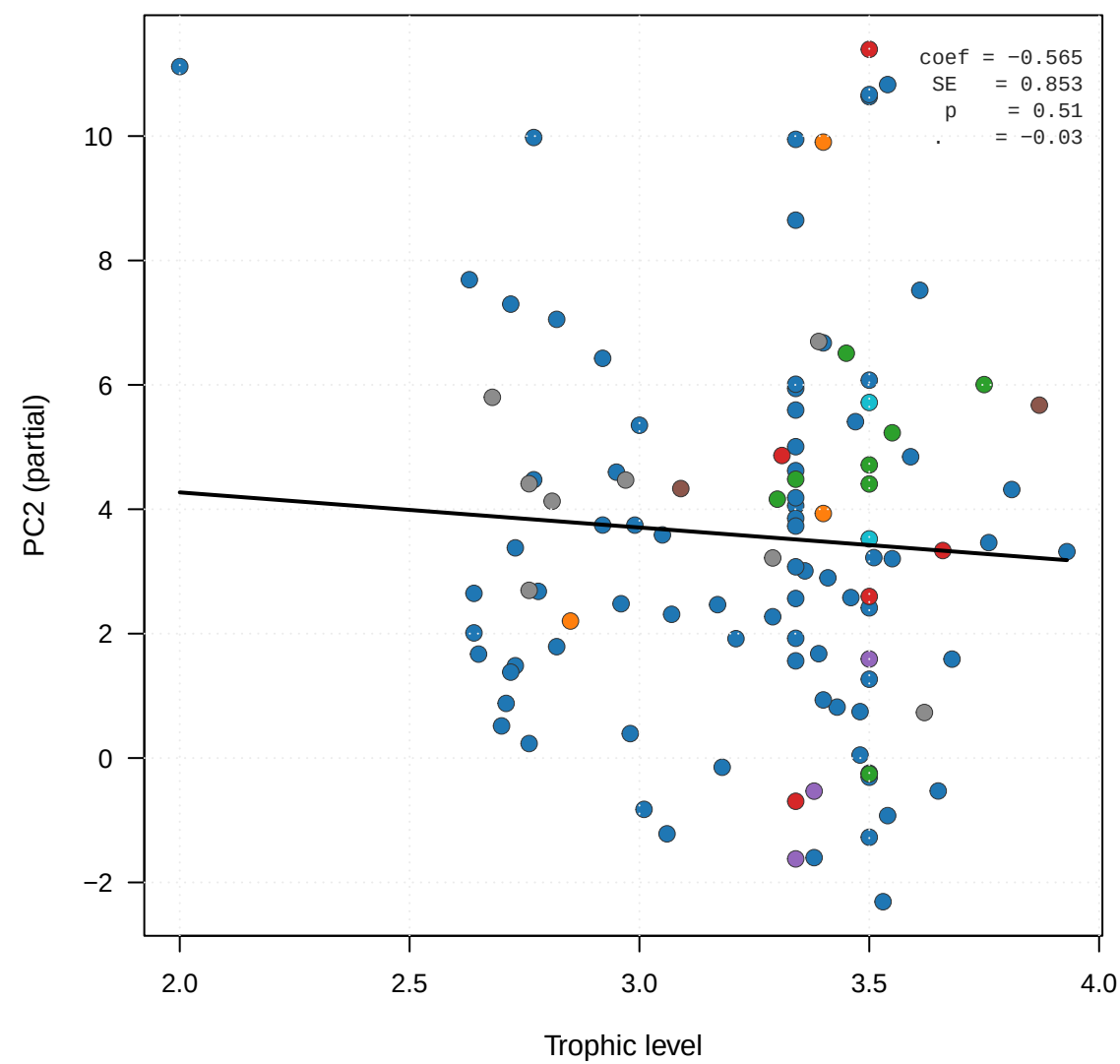
PC2 vs Trophic level
