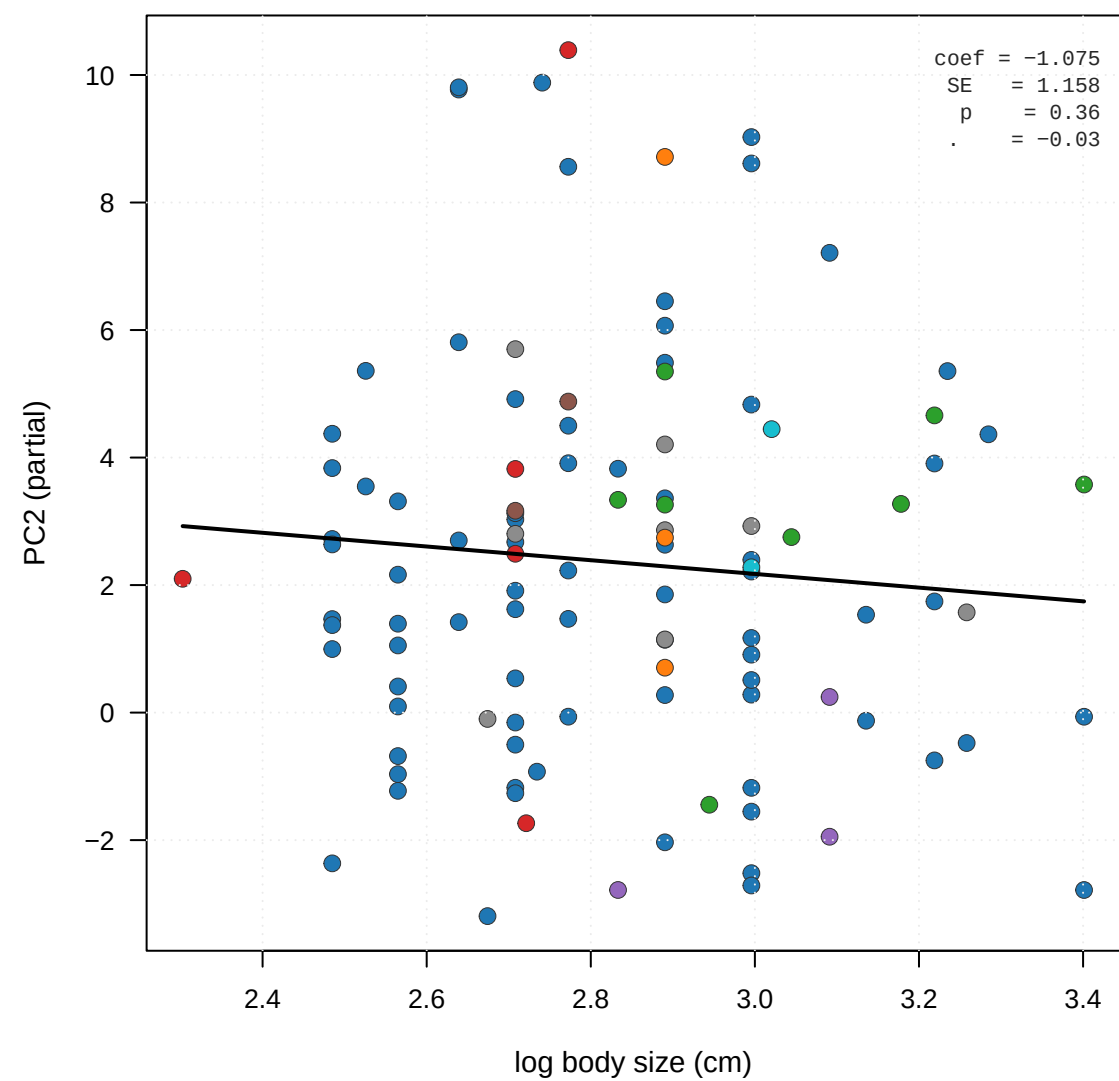
PC2 vs log body size (cm)
