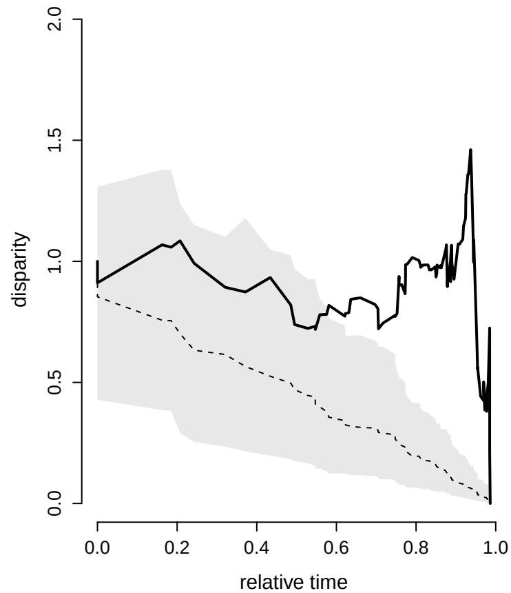
PC2 (MDI = 0.4673)
