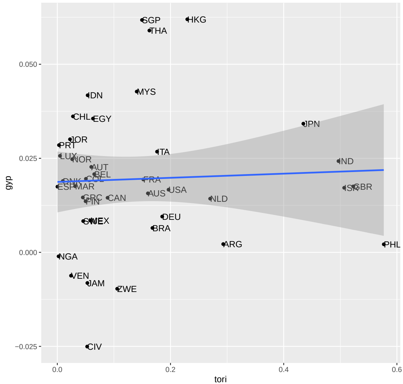
Bivariate regression
