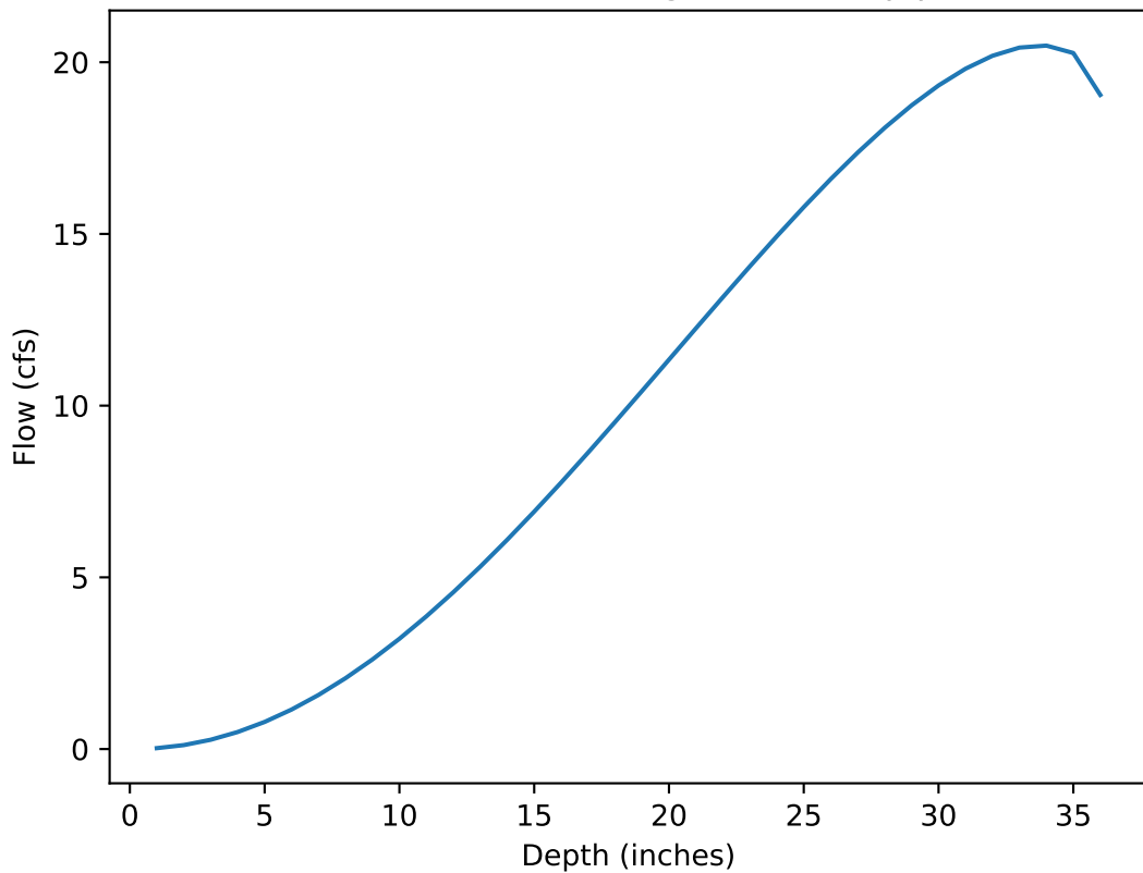
Flow in 36 inch corrugated metal pipe
