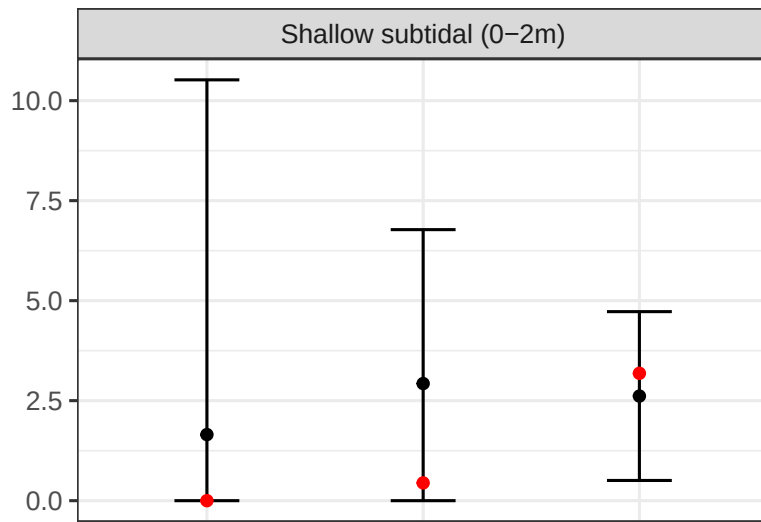
Predicted Mean Seagrass Cover
