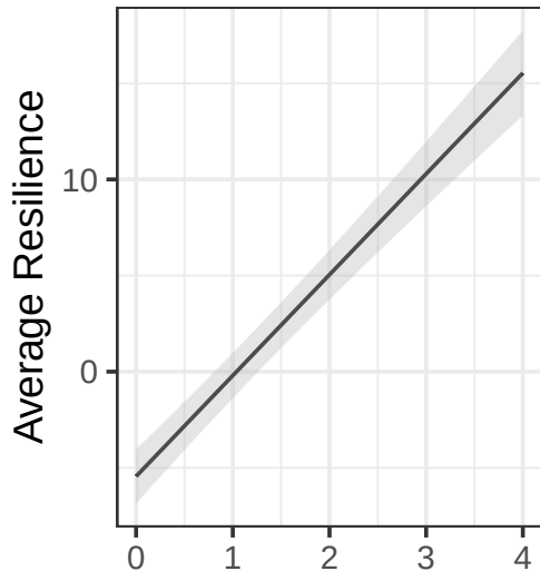
Species Richness
