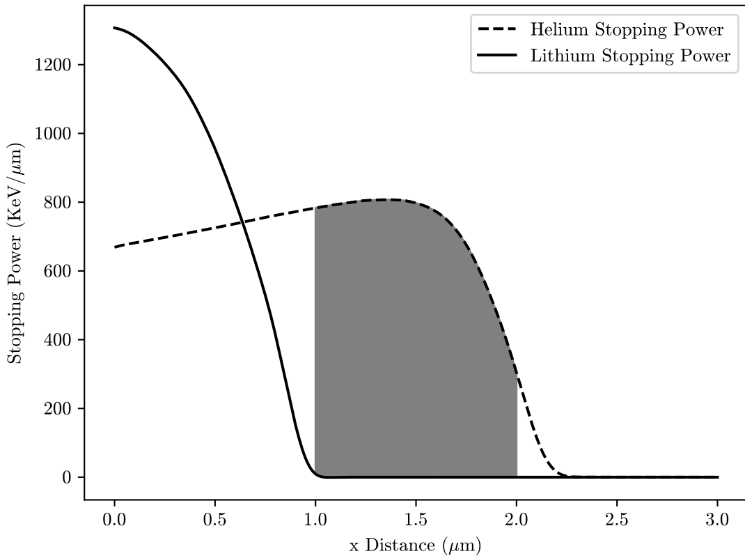
Stopping Power of emitted He, Li in Junction
