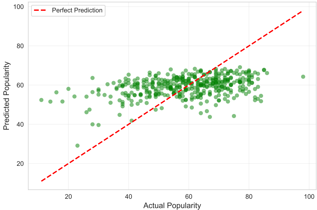
Random Forest ( R^2 = 0.141 )
