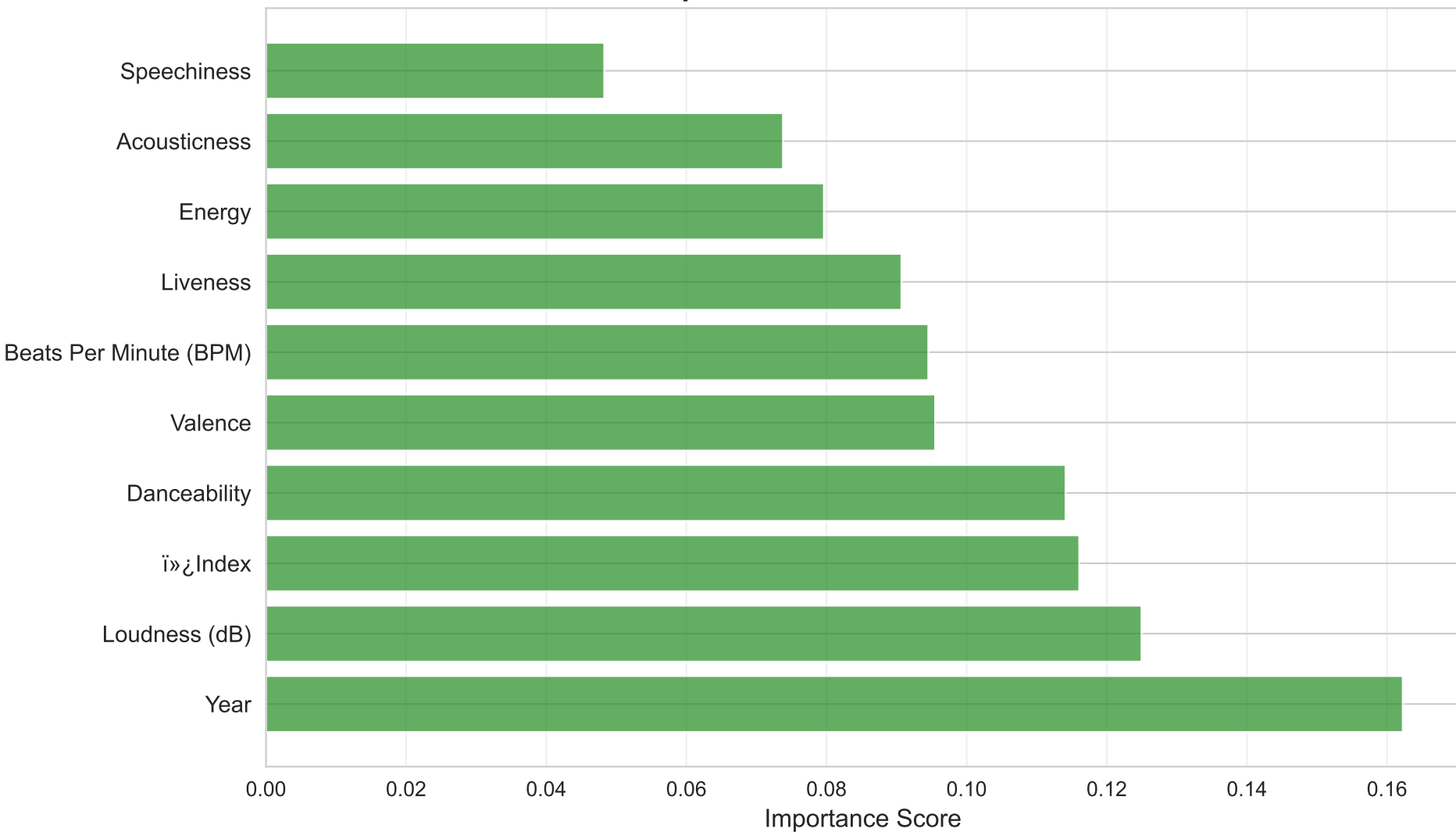
Feature Importance from Random Forest Model
