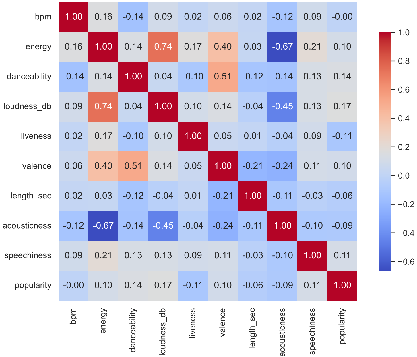
Correlation Between Audio Features and Popularity
