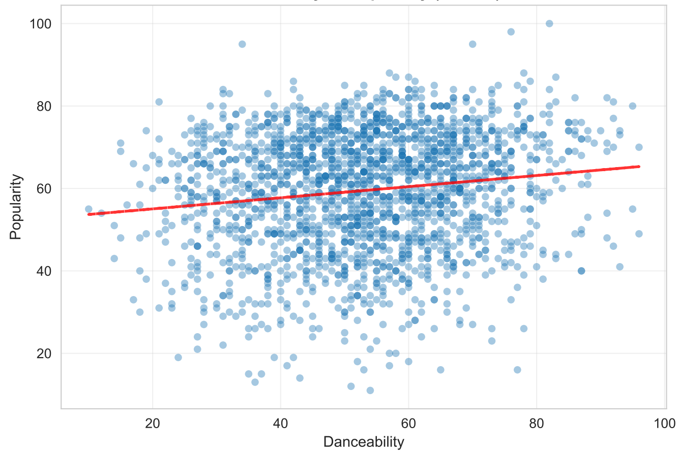
Danceability vs Popularity ( r=0.144 )
