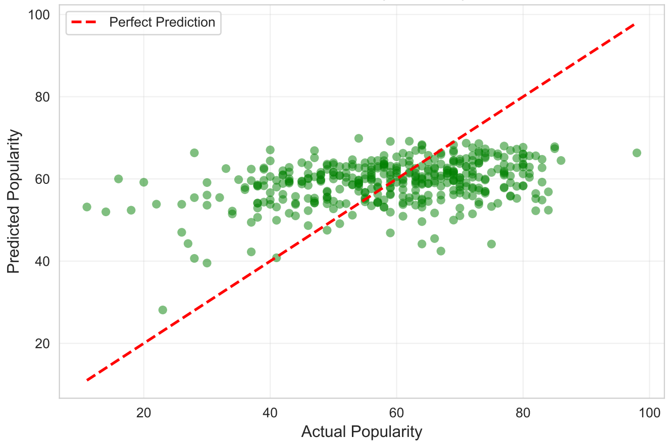
Random Forest ( R^2 = 0.131 )
