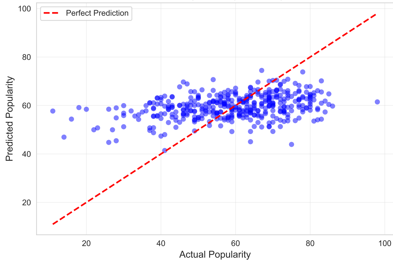
Linear Regression ( R^2 = 0.121 )
