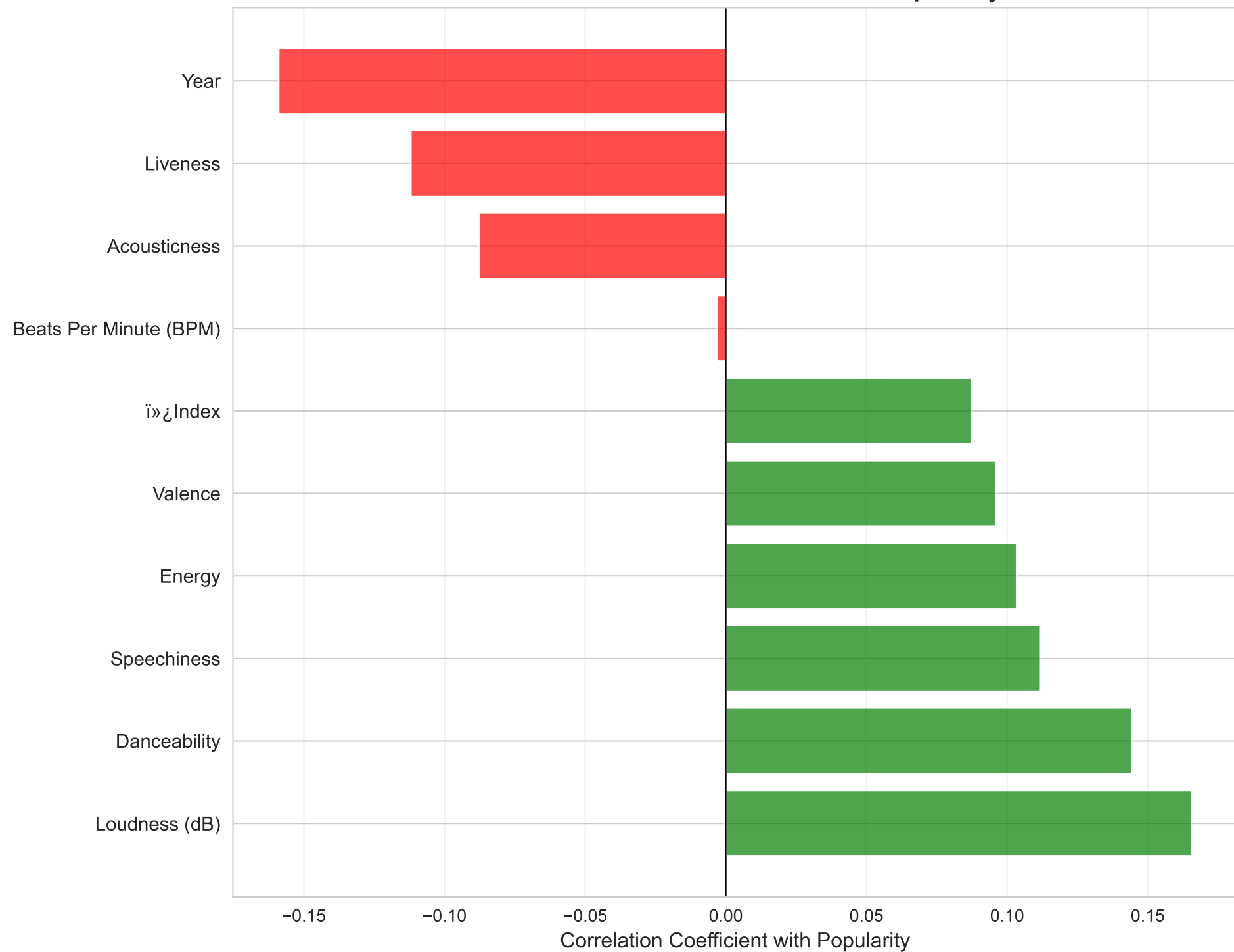
How Audio Features Correlate with Popularity
