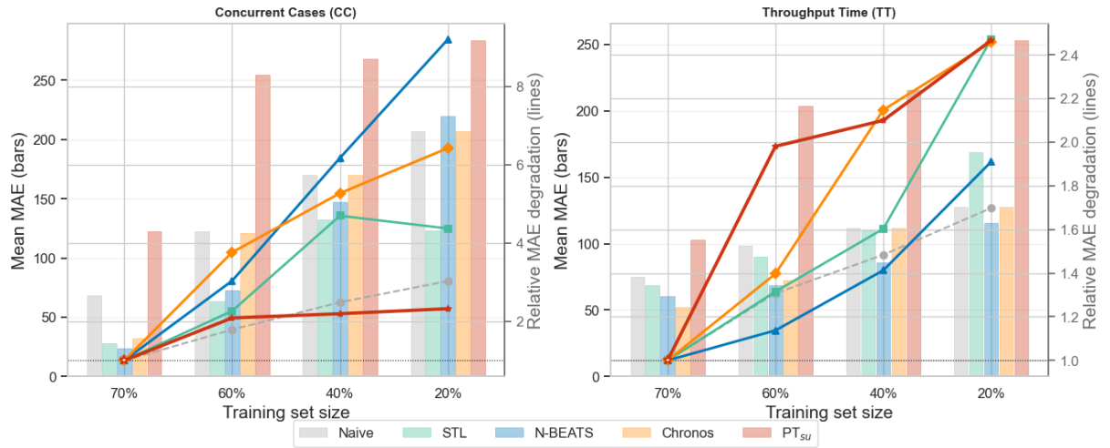
Figure 1: Sensitivity of different approaches to training data size, averaged over all synthetic LoAp logs. Bars show absolute MAE per approach for varying training set sizes. Lines show the relative degradation of the approaches w.r.t. their original performance when the full training set (70%) is given.
