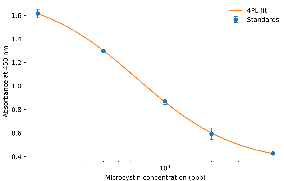
Microcystin-ADDA ELISA standard curve
