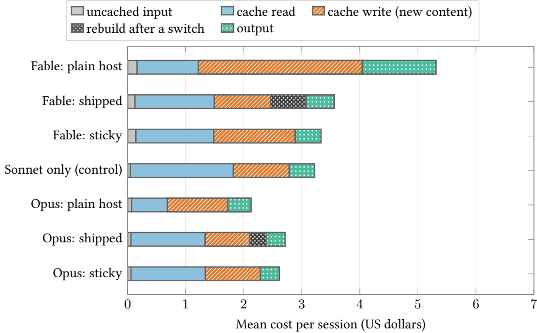
Figure 16: Mean cost per session, split by what was paid for (all splits, cost-valid sessions, tools-normalized). “Rebuild after a switch” is the extra paid for re-writing history to a new model’s cache.
