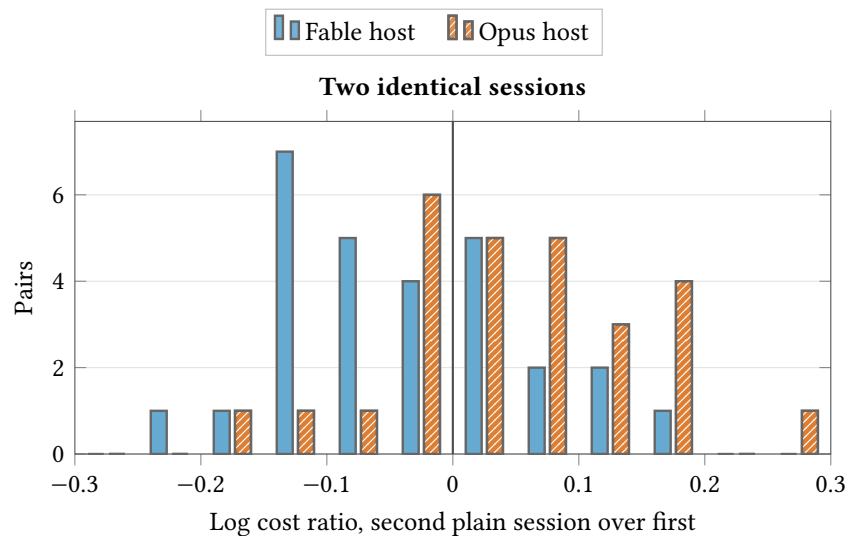
Figure S28: Two identical sessions differ by chance; this spread is the noise floor. Distribution of the log cost ratio between two identical plain-host sessions (A/A), by host.
