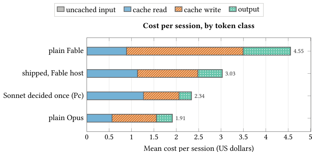
Figure S38: Plain Fable spends most of its money writing to the cache. Mean cost per S1 session split by token class, at the study's price table (exploratory).
