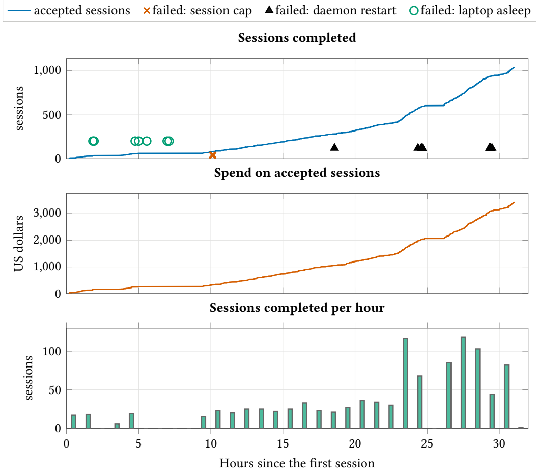
Figure S4: The campaign ran in bursts separated by pauses, with one burst of failed attempts. Campaign progress reconstructed from the data: accepted sessions completed and their spend over the 31.1 hours from the first session to the last, sessions completed per hour, and when failed attempts started, by cause.
