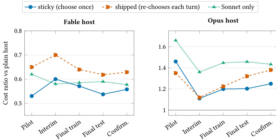
Figure S19: The Fable estimates were right from the pilot onwards; the Opus estimates moved as evidence accumulated. Cost ratio of each routed arm as the evidence accumulated: the screening pilot, the interim dashboard during the run (partial training data), the final training and test splits (all cost-valid pairs) and the confirmatory test result (pair reading).
