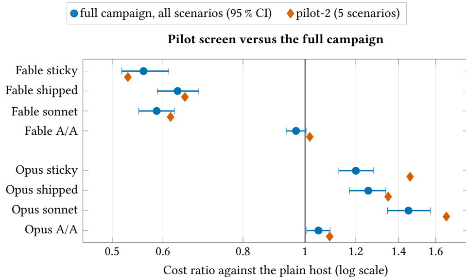
Figure S3: A five-scenario pilot found the direction of the routing effect, not its size. The second screening pilot (40 pairs on 5 scenarios) against the full campaign (all scenarios, 95 % intervals), for each arm and host. The first pilot was a smoke test of the harness ($43.72) whose rows were not packaged.
