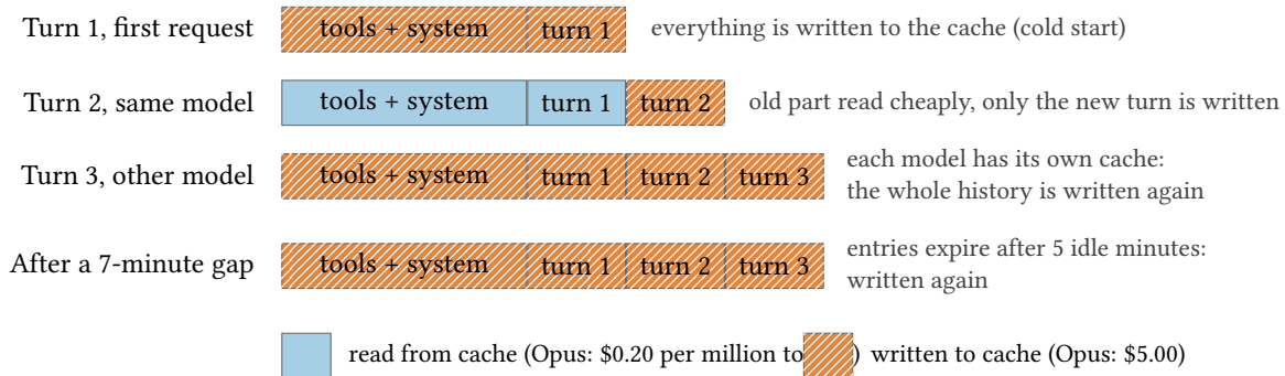
Figure S20: Within one model only the new turn is written to the cache; a switch of model or effort rewrites everything. How the prompt cache behaves over a conversation (schematic, not to scale).
