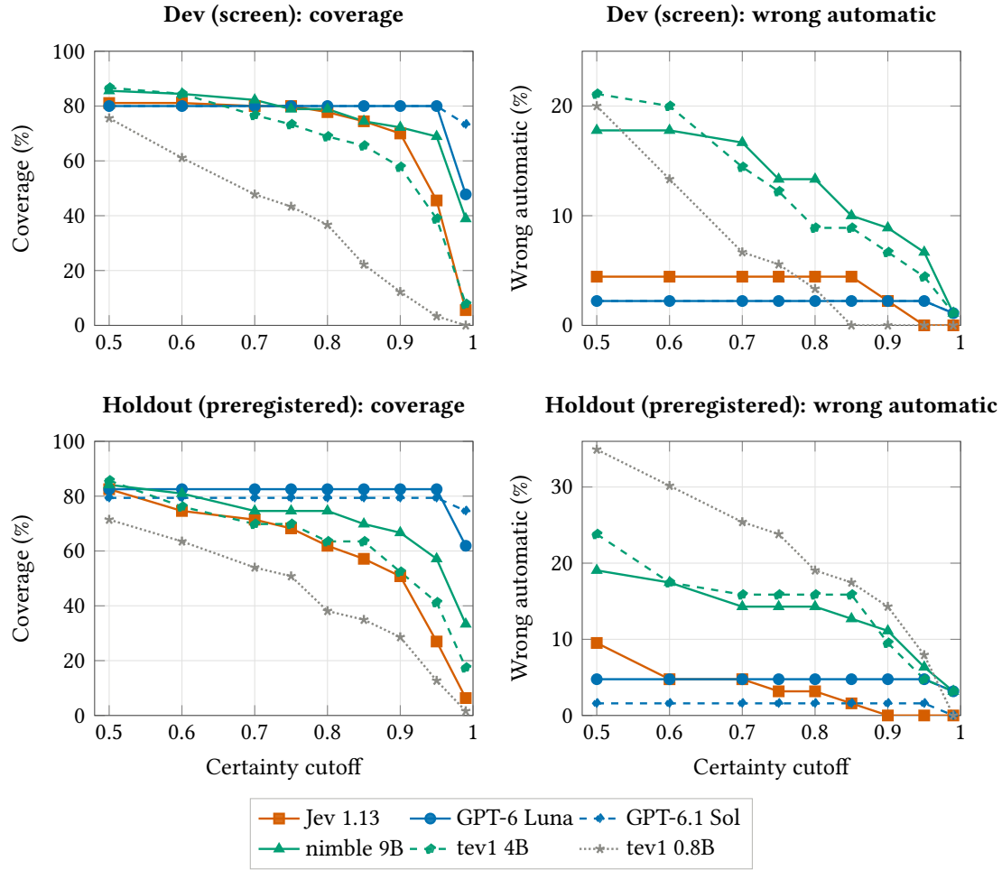
Figure S9: Raising the certainty cutoff always lowers coverage, but lowers wrong automatic actions only for judges whose confidence is informative. Threshold sweep. Left: coverage; right: wrong-automatic rate, as the certainty cutoff rises from 0.5 to 0.99. Top: dev [screen]; bottom: holdout [preregistered]. Per-case majorities over repetitions.
