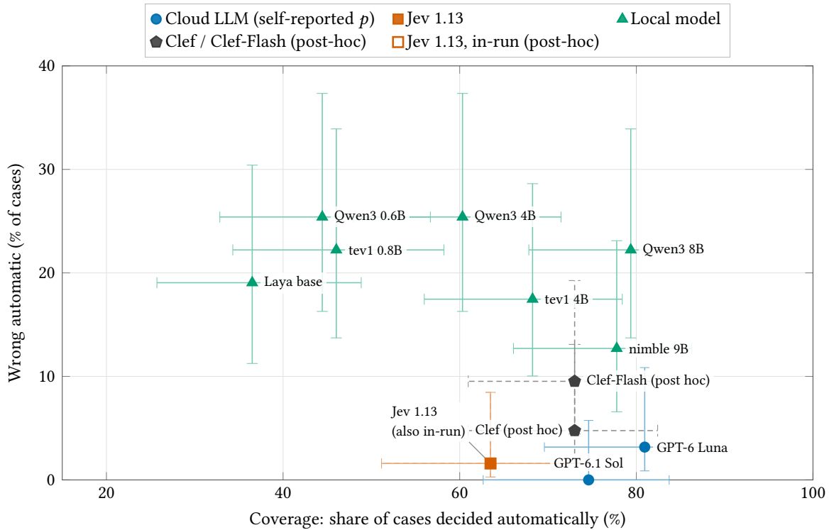
Figure S10: The cloud judges and Jev rarely act wrongly; the local models misfire more. Wrong-automatic rate against coverage on the holdout: the safety–usefulness trade-off of each judge, with the post-hoc Clef arms.
