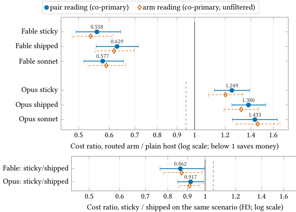
Figure S14: On the main-v1 test split, every Fable routing arm saved money and every Opus arm cost more. Confirmatory cost ratios on the main-v1 test split. Top: each routed arm against the plain host. Bottom: the sticky arm against the shipped arm on the same scenarios. Whiskers are 95 % intervals; the dashed lines mark preregistered thresholds.
