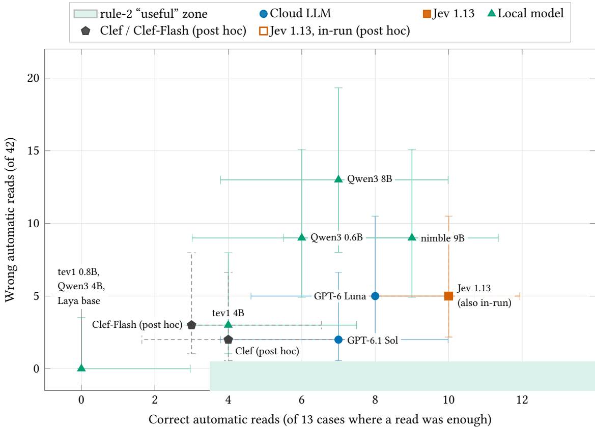
Figure S6: On real read decisions, no judge reached the usefulness zone. Real decisions: correct automatic reads against wrong automatic reads on trace-holdout, with 95 % Wilson intervals: the preregistered run, plus the post hoc Clef arms (black pentagons). The shaded strip is where the preregistered rule would call a judge useful.
