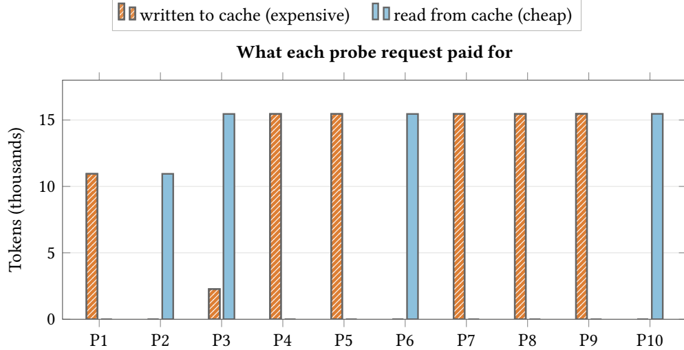
Figure S21: A request reuses the cache only with the same key, model and effort, within the cache lifetime. The probe requests of Table S54 , drawn: tokens written and read by each.
