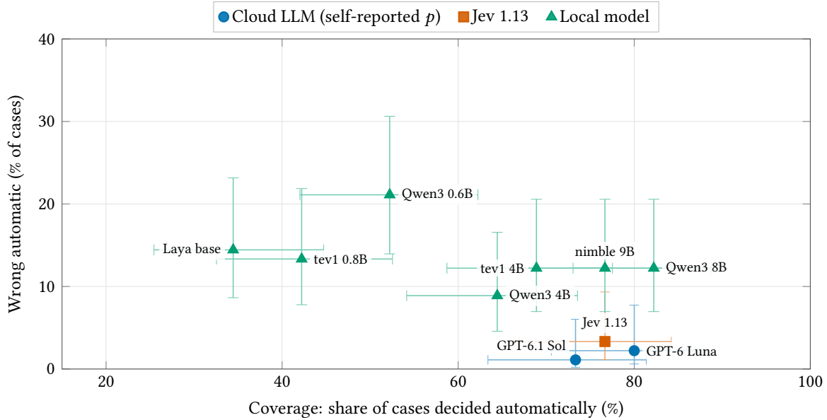
Figure S8: The safety–usefulness trade-off of every judge on the dev split [screen]: the best judges sit low and to the right. Wrong automatic rate against coverage on the dev split [screen]. Whiskers are 95 % Wilson intervals in both directions. Marker shape and colour show the judge family.
