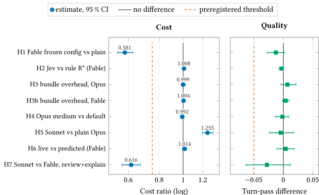
Figure S33: Two hypotheses carry money (H1, H5); the rest are guards. S1 hypotheses H1–H7: cost ratio (left, log scale) and turn-pass difference (right), each with its 95 % interval. H3b is descriptive. Thresholds: the H1 cost bound (0.75) and the quality margin ( -0.05 ).
