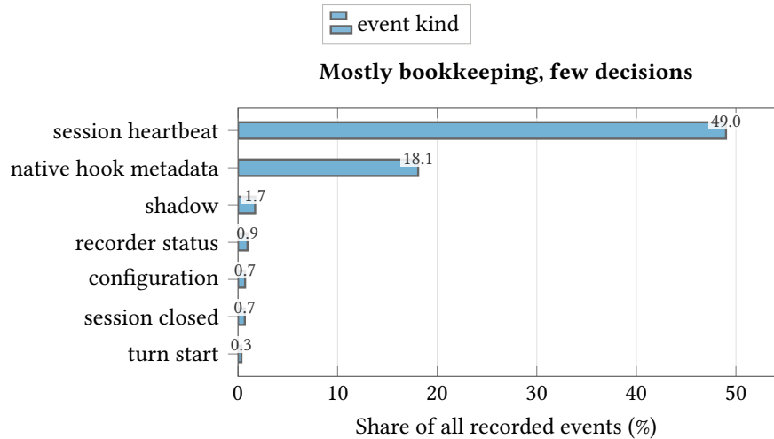
Figure S32: Most recorded events are bookkeeping; decision-bearing events are a thin slice. What the observatory store holds: the seven most common kinds of recorded event, as a share of all events.
