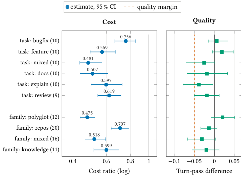
Figure S35: Every subgroup saves money; quality intervals for several subgroups are too wide to rule out a loss. Lower bounds fall below the -0.05 margin for the explain ( -0.078 ), mixed ( -0.071 ) and docs ( -0.069 ) tasks and the mixed ( -0.067 ) and knowledge ( -0.056 ) families; review’s lower bound is -0.050 . Subgroups hold 9–20 scenarios; treat as hypothesis-generating. The frozen Fable configuration against plain Fable, split by task type and by scenario family (number of cost-valid scenarios in brackets; the quality panel is unfiltered and uses every scenario of the subgroup), with 95 % intervals. Exploratory: subgroups were not preregistered except H7.
