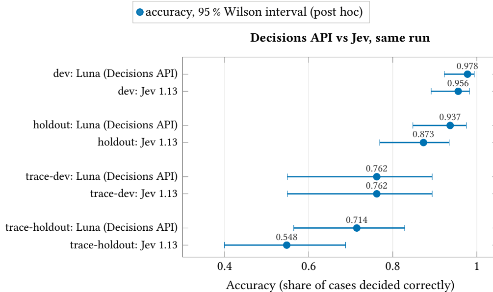
Figure S7: The Decisions API was at or above Jev on every split (post hoc). OpenAI Decisions API (GPT-6 Luna) against the in-run Jev reference: per-case majority accuracy with 95 % Wilson intervals on the four splits (post hoc).
