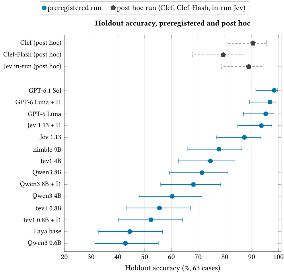
Figure S5: No accuracy difference between the top judges was detected after the preregistered correction. Holdout accuracy with 95 % Wilson intervals: the preregistered run, then (above the gap) the post hoc run of Clef, Clef-Flash and the in-run Jev reference.
