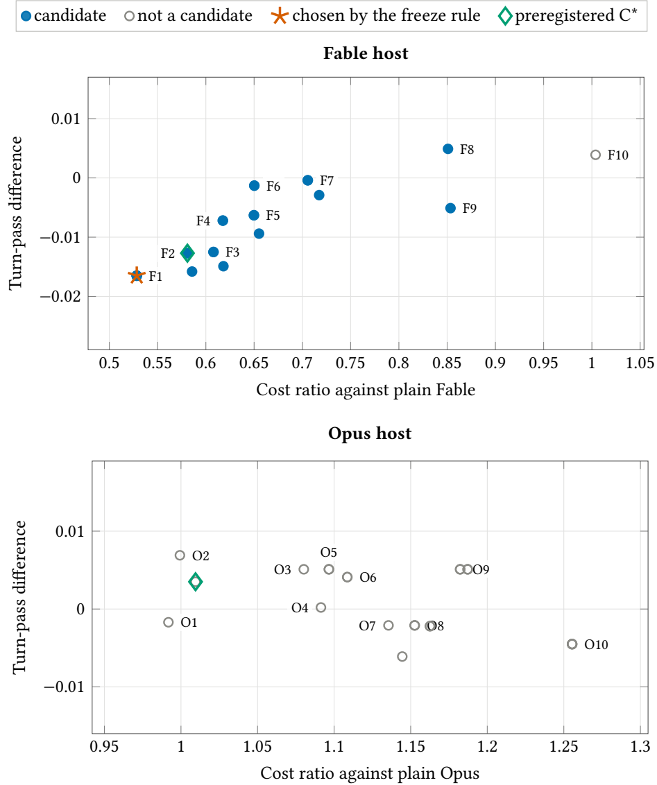
Figure S36: On Fable many configurations qualify; on Opus none does. All 23 Fable and 23 Opus configurations the freeze rule considered: cost ratio against the host’s plain default and turn-pass difference (point estimates). Keys group configurations that land on the same point; Table S74 lists them.
