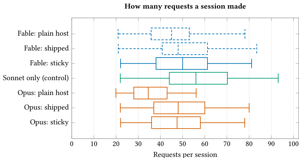
Figure S29: Sonnet-heavy sessions made more requests for the same scripted work. Main-loop requests per session by kind of session: box from the 25th to the 75th percentile, line at the median, whiskers from the 5th to the 95th percentile.
