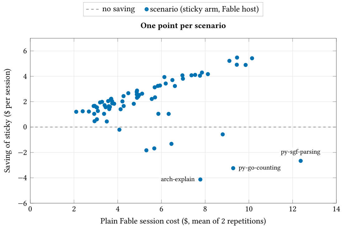
Figure S27: Most scenarios saved money on Fable, and expensive scenarios tended to save more. Scenario by scenario: the mean plain Fable cost against the mean saving of the sticky arm (Fable host). The three scenarios where sticky cost the most extra are labelled.
