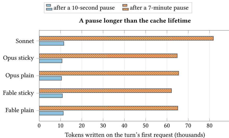
Figure S25: After a long pause the first request rewrites the history on every arm and host. Cache-write tokens on the first request of a turn, after a short pause and after a long pause (turns 2 onwards), per arm and host.
