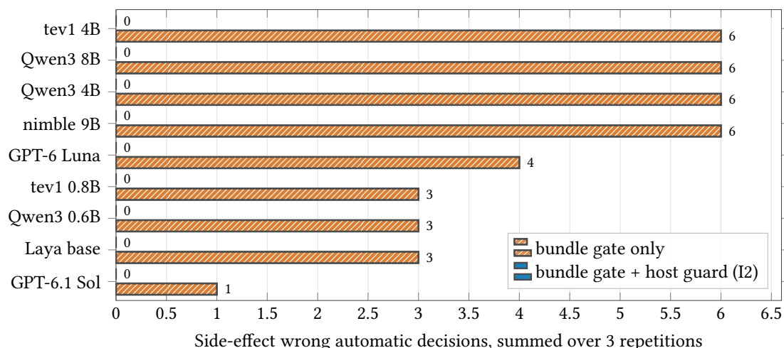
Figure S31: The host guard removed every side-effect wrong automatic action, at a small cost in coverage. The host guard (I2) on the holdout [preregistered]: side-effect wrong automatic decisions per judge, summed over repetitions, without and with the guard.
