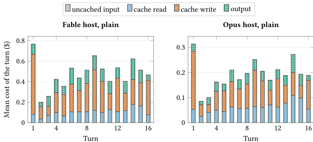
Figure S24: Turn 1 is mostly cache writes; later turns are mostly cache reads. What each turn of a plain-host session paid for, by turn index (mean dollars per token class).
