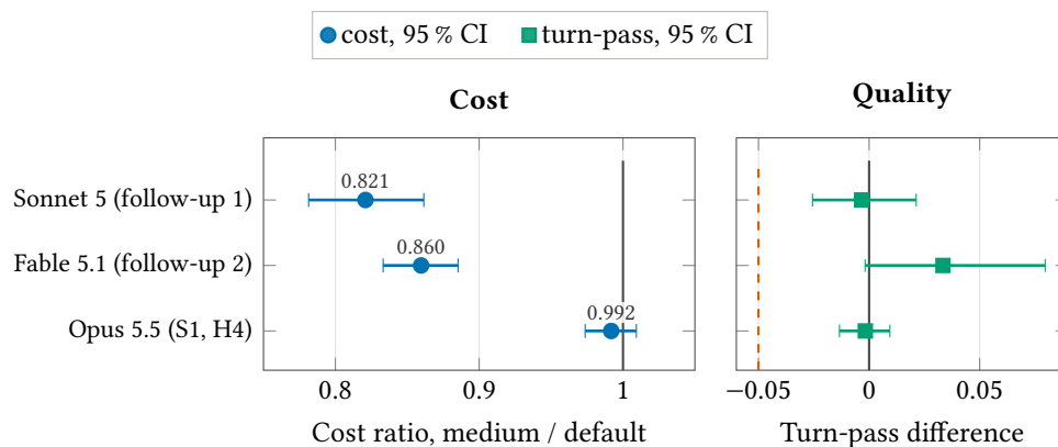
Figure S37: Medium effort saved money on Sonnet and Fable but did not demonstrate a saving on Opus. Medium against default reasoning effort, measured in three studies: Sonnet (follow-up 1), Fable (follow-up 2) and Opus (S1, H4). 95 % intervals.
