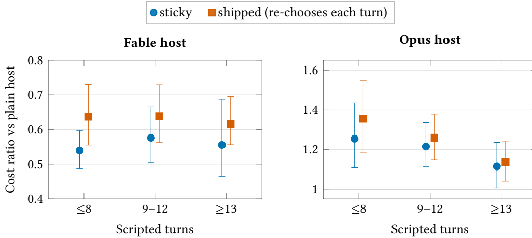
Figure S30: The routing ratio barely depended on scripted session length. Cost ratio by scripted session length, all splits, with 95 % intervals.
