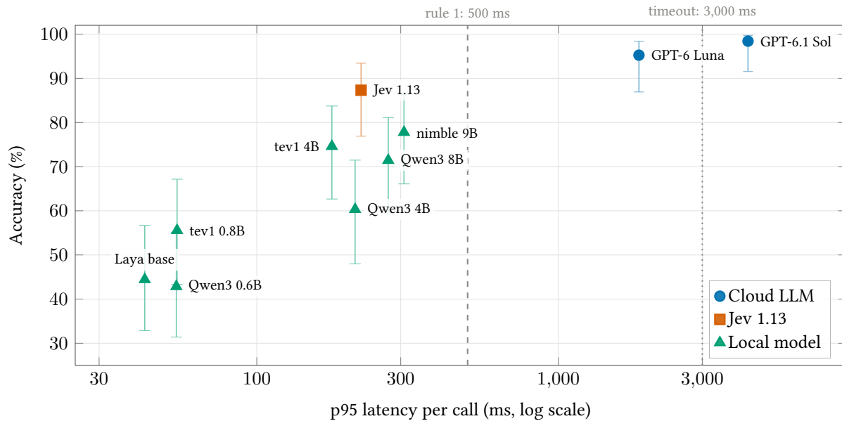
Figure 4: Accuracy against p95 latency (log scale) on the holdout [preregistered] , with 95 % Wilson intervals on accuracy. The dashed line is rule 1’s 500 ms bar; the dotted line is the bundle’s 3 s timeout.
