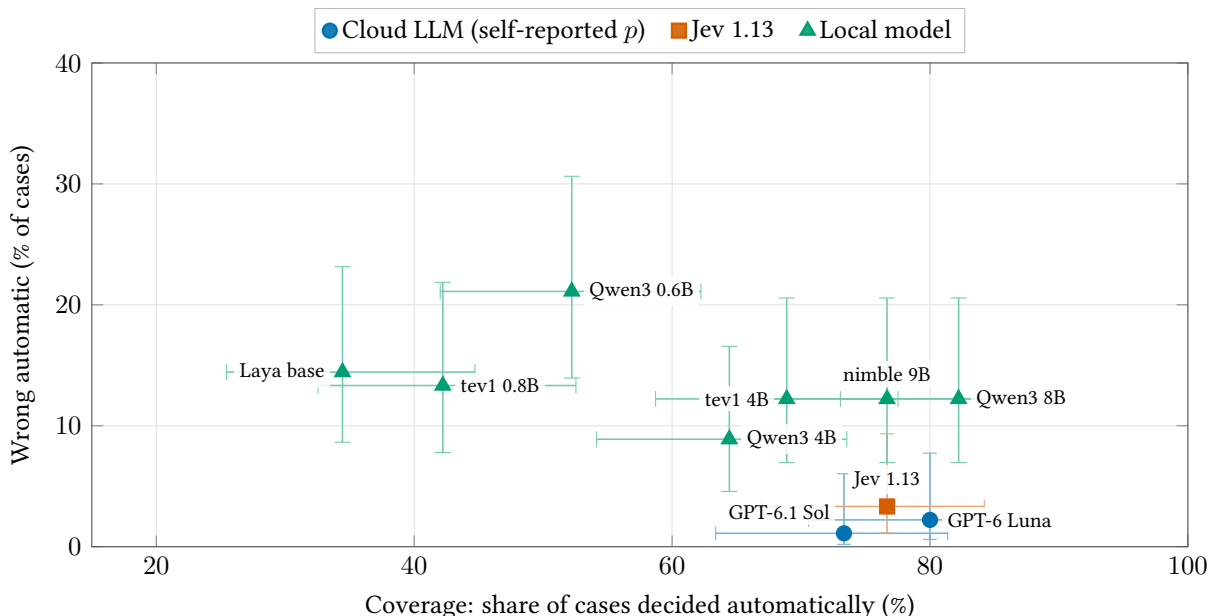
Figure 1: Wrong automatic rate against coverage on the dev split [screen]. Whiskers are 95 % Wilson intervals in both directions. Marker shape and colour show the judge family.
