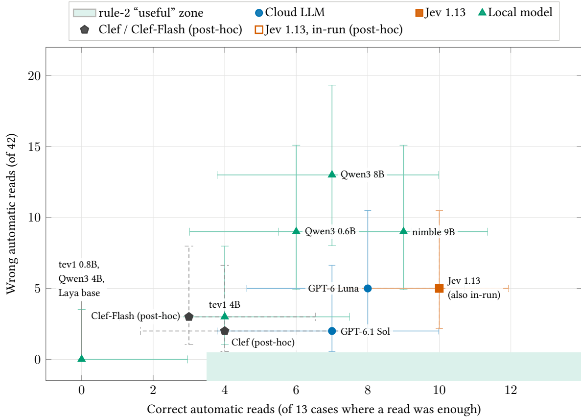
Figure 6: Real decisions: correct automatic reads against wrong automatic reads on trace-holdout, with 95 % Wilson intervals: the preregistered run, plus the post-hoc Clef arms (black pentagons). The shaded strip is where the preregistered rule would call a judge useful.
