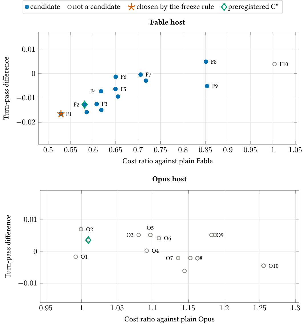
Figure 13: All 23 Fable and 23 Opus configurations the freeze rule considered: cost ratio against the host’s plain default and turn-pass difference (point estimates). Keys group configurations that land on the same point; Table 7 lists them.
