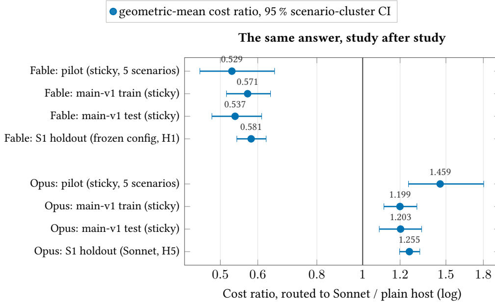
Figure 16: Routing to Sonnet against the plain host, per host, across the pilot, the main-v1 training and test splits and S1. Main-v1 rows are the sticky arm without the quality filter; the S1 rows are H1 (Fable) and H5 (Opus).
