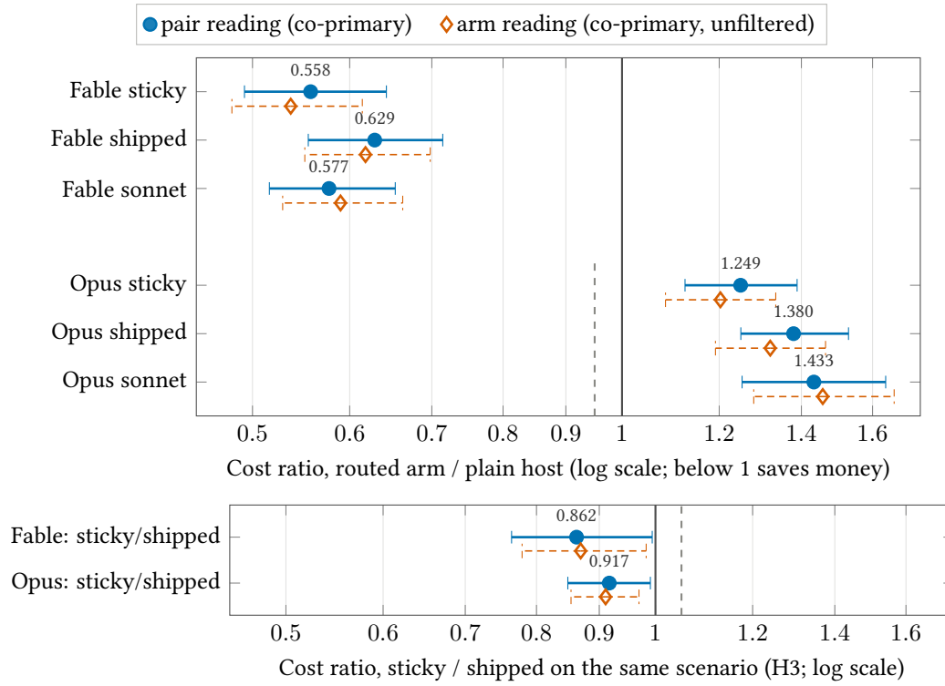
Figure 8: Confirmatory cost ratios on the main-v1 test split. Top: each routed arm against the plain host. Bottom: the sticky arm against the shipped arm on the same scenarios. Whiskers are 95 % intervals; the dashed lines mark preregistered thresholds.
