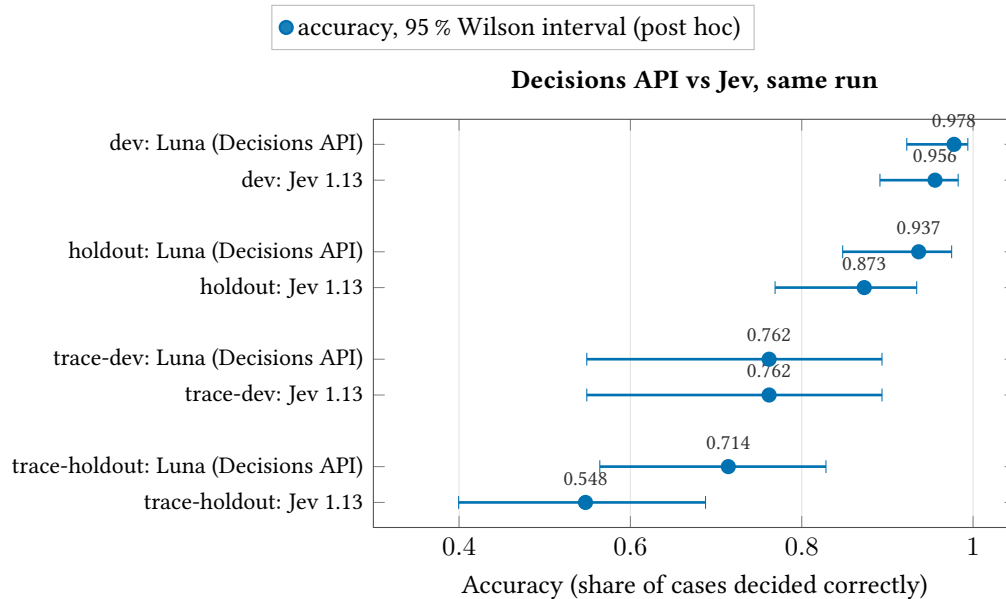
Figure 7: OpenAI Decisions API (GPT-6 Luna) against the in-run Jev reference: per-case majority accuracy with 95 % Wilson intervals on the four splits (post hoc).
