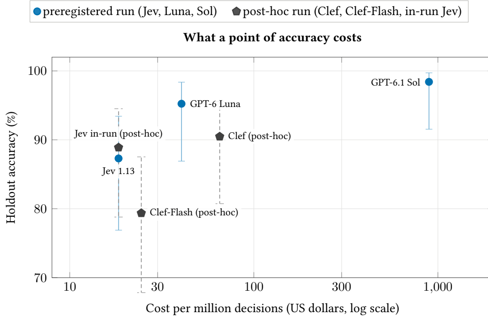
Figure 5: Cost per million decisions (log scale) against holdout accuracy, for the judges that have a price. Blue: preregistered run; black pentagons: post-hoc run (Clef, Clef-Flash and the in-run Jev reference).
