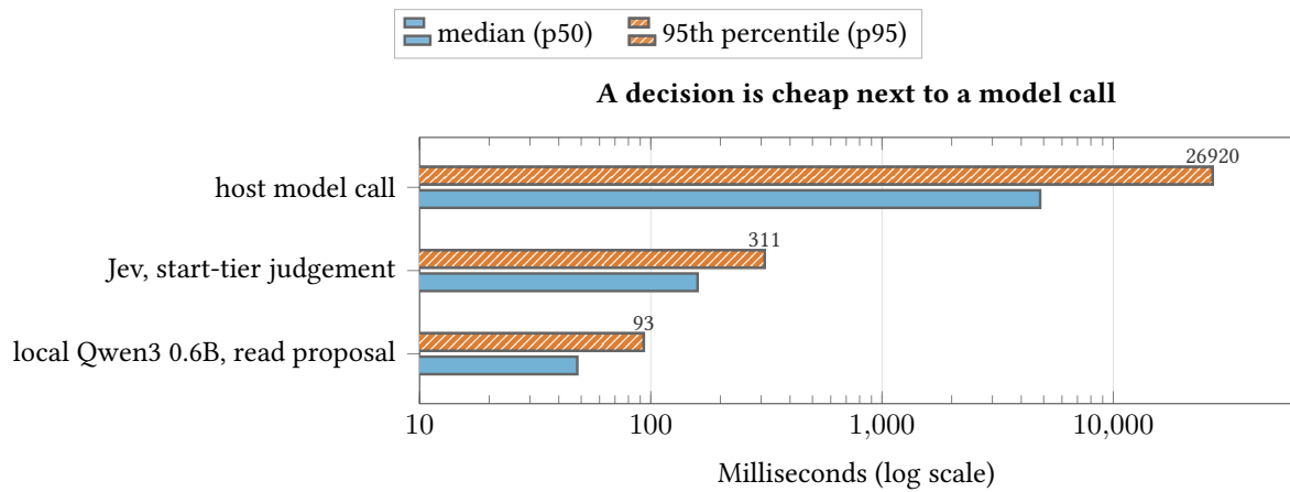
Figure 2: Latency of decision calls and of host model calls, measured by the bundle’s recorder (log scale).
