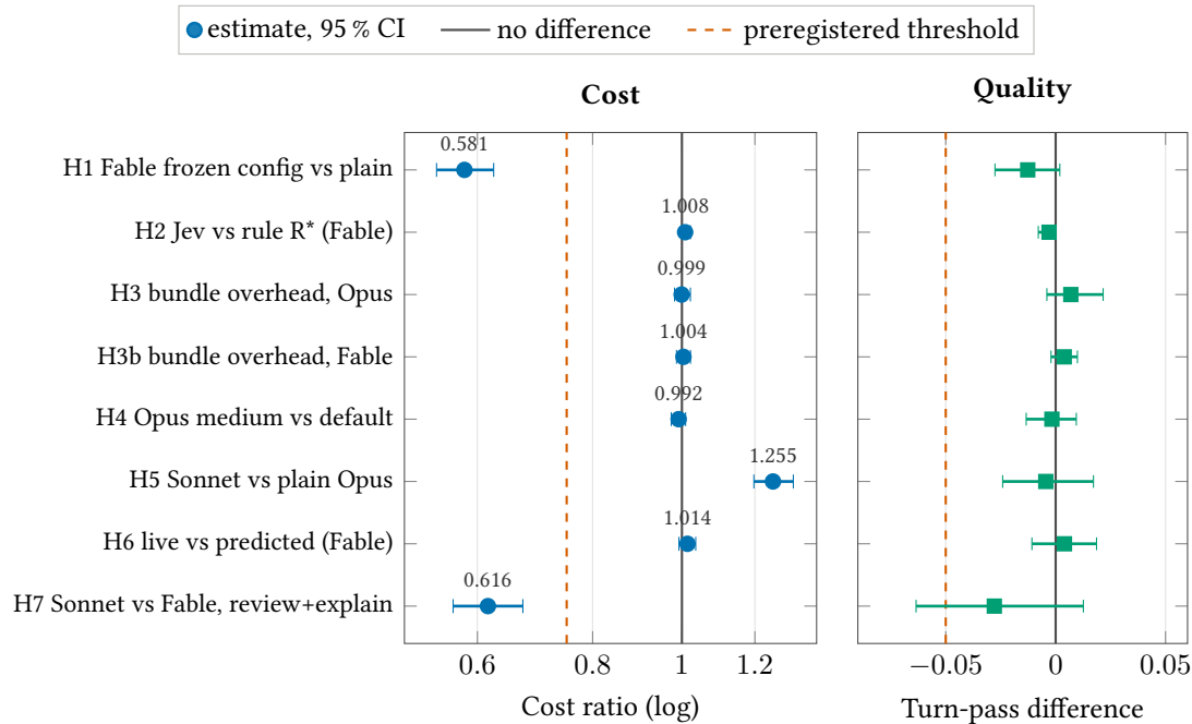
Figure 10: S1 hypotheses H1–H7: cost ratio (left, log scale) and turn-pass difference (right), each with its 95 % interval. H3b is descriptive. Thresholds: the H1 cost bound (0.75) and the quality margin (−0.05).
