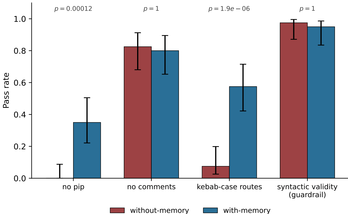
Per-constraint pass rates with 95% Wilson CIs ( N = 40 )
