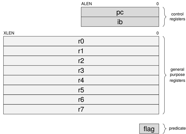
Figure 1.20.: register state accessible by 16-bit instruction packet.
