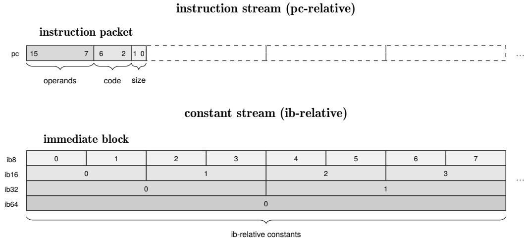
Figure 1.19.: program counter and immediate base register.
