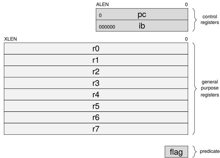
Figure 1.12.: register state accessible by 16-bit instruction packet.
