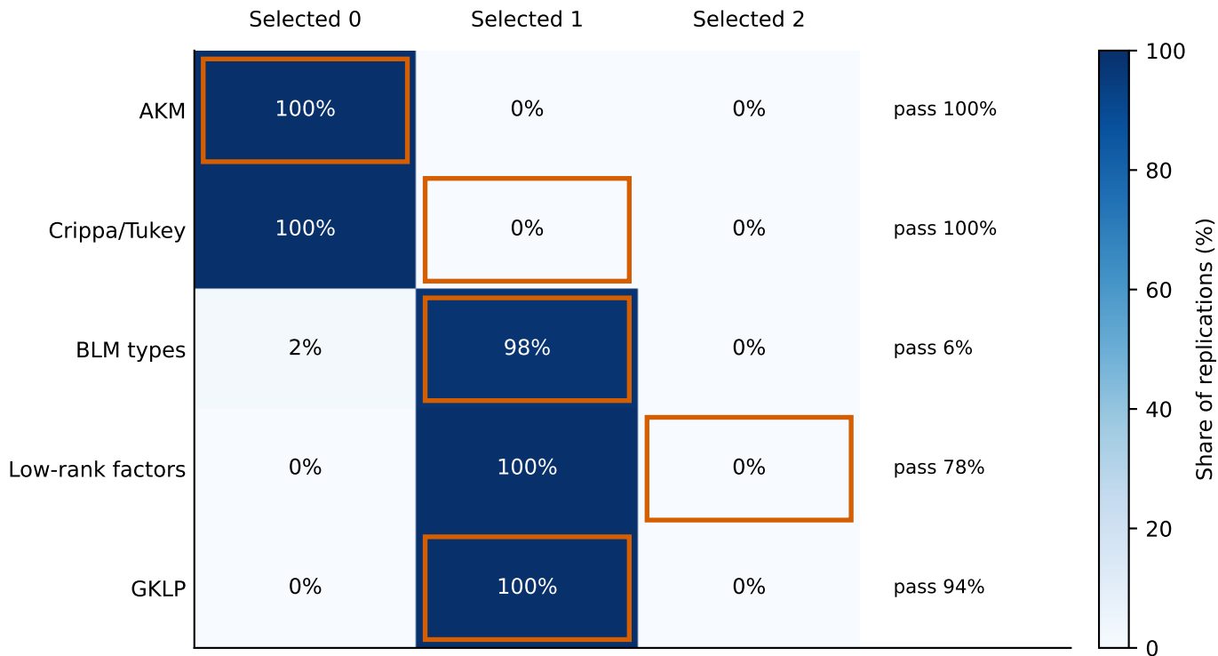
BIC rank selection; orange box marks the true rank
