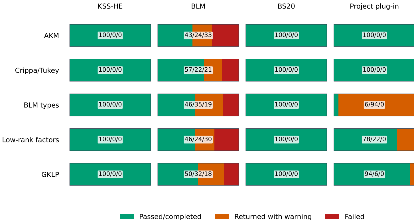
Estimator status in 100 replications (pass / warning / failure)
