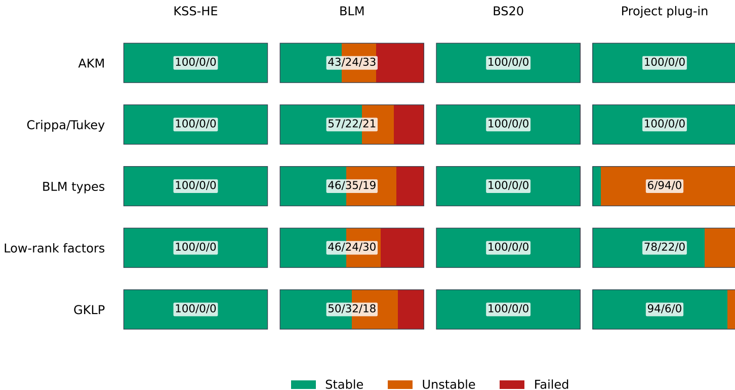
Estimator status in 100 replications (stable / unstable / failed)
