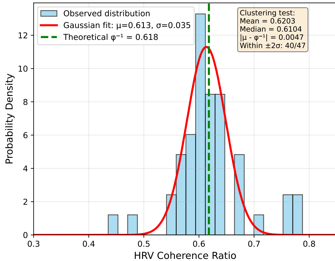
Coherence Distribution (N=47)
