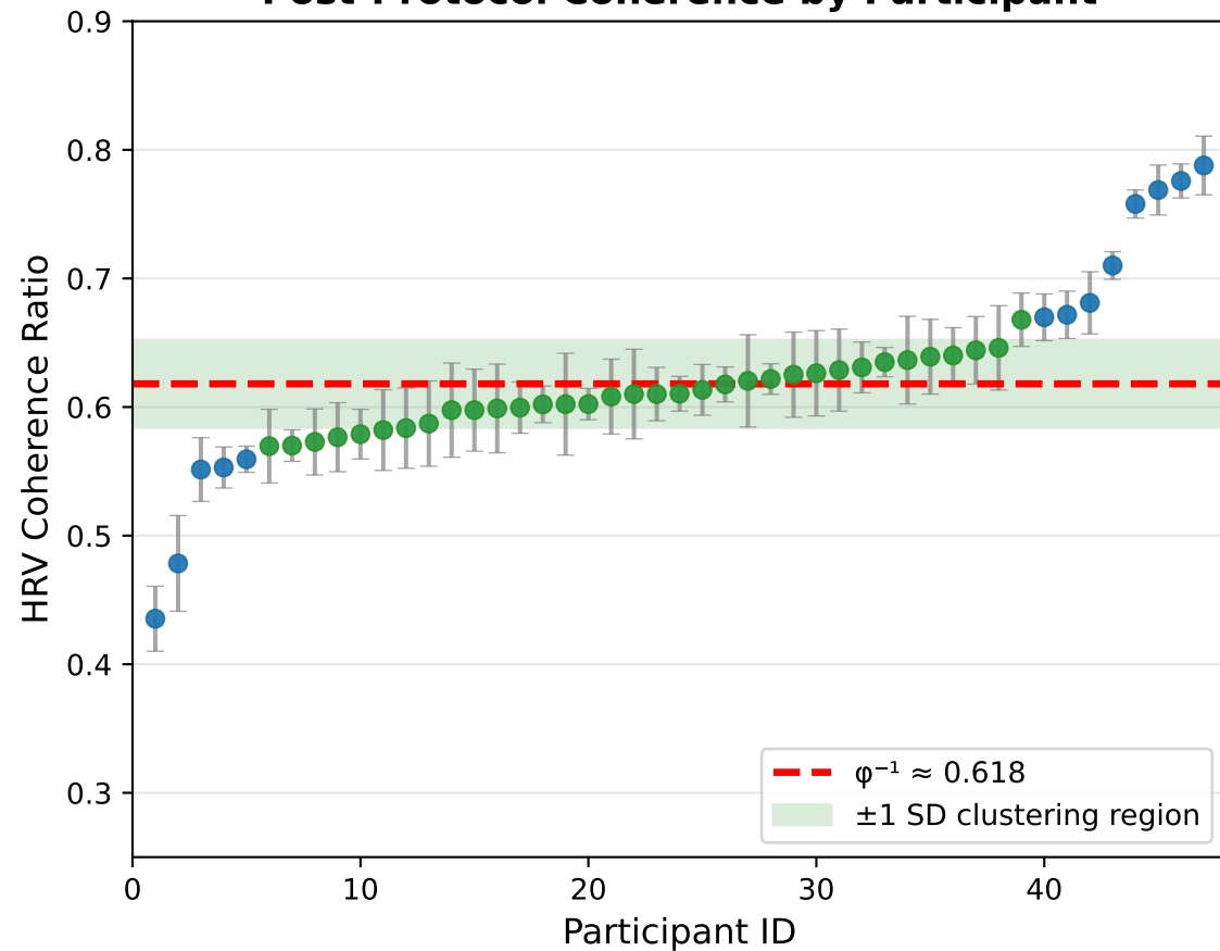
Post-Protocol Coherence by Participant
