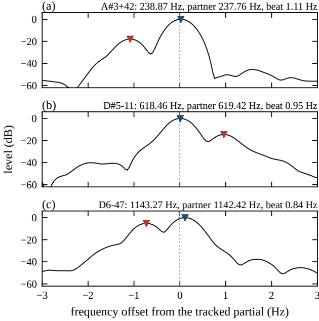
Figure 5: Zoom spectra of the three lower partials of the recorded bowl over their core intervals ( T = 4.5 to 4.7 s). Blue: main mode, red: partner; dashed: the frequency tracked from the frames.
