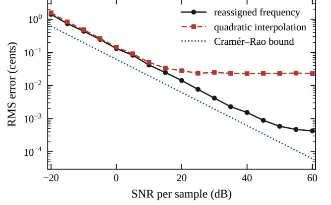
Figure 3: Single-frame frequency error for a sinusoid near 1 kHz in white noise ( N = 8192 , f_s = 48 kHz; 1 cent is 0.58 Hz here), against the Cramér–Rao bound [27].
