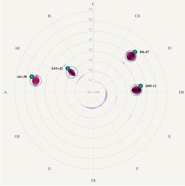
Figure 1: The spiral display for the recorded bowl of Section 9.3: reassigned spectrum of the window 18.62–23.80s (display range 60dB) and the four listed partials, numbered as in Table 1. One turn is one octave, from C2 at the centre to C9; equal-tempered pitch classes lie on the radial lines.
