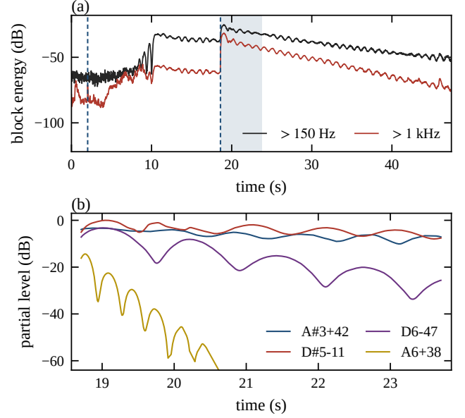
Figure 4: Recorded bowl. (a) Block energies of the onset detector over the whole recording; dashed: detected attacks; shaded: the selected window. (b) Peak levels of the four listed partials in the window, relative to the strongest; the periodic dips are beats.
