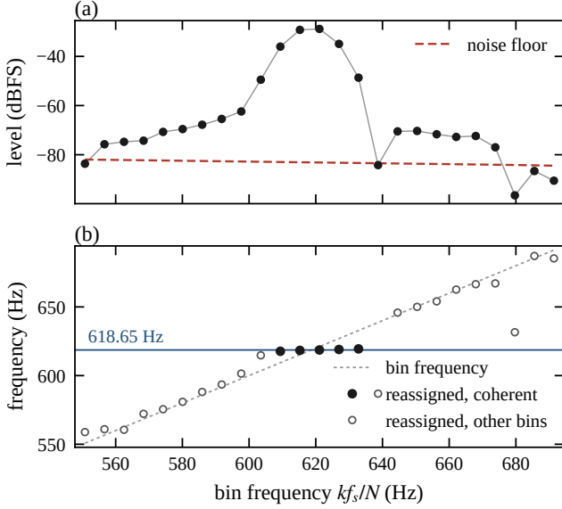
Figure 2: One frame of the recorded bowl of Section 9.3 ( t = 20.21 s) around the partial D#5-11. (a) Bin levels and noise floor. (b) Reassigned frequency of each bin; filled: bins within 0.45 bin of the peak’s value. The single-frame value, 618.65 Hz, differs from the window estimate, 618.46 Hz, because the partial is a beating pair (Fig. 5b).
