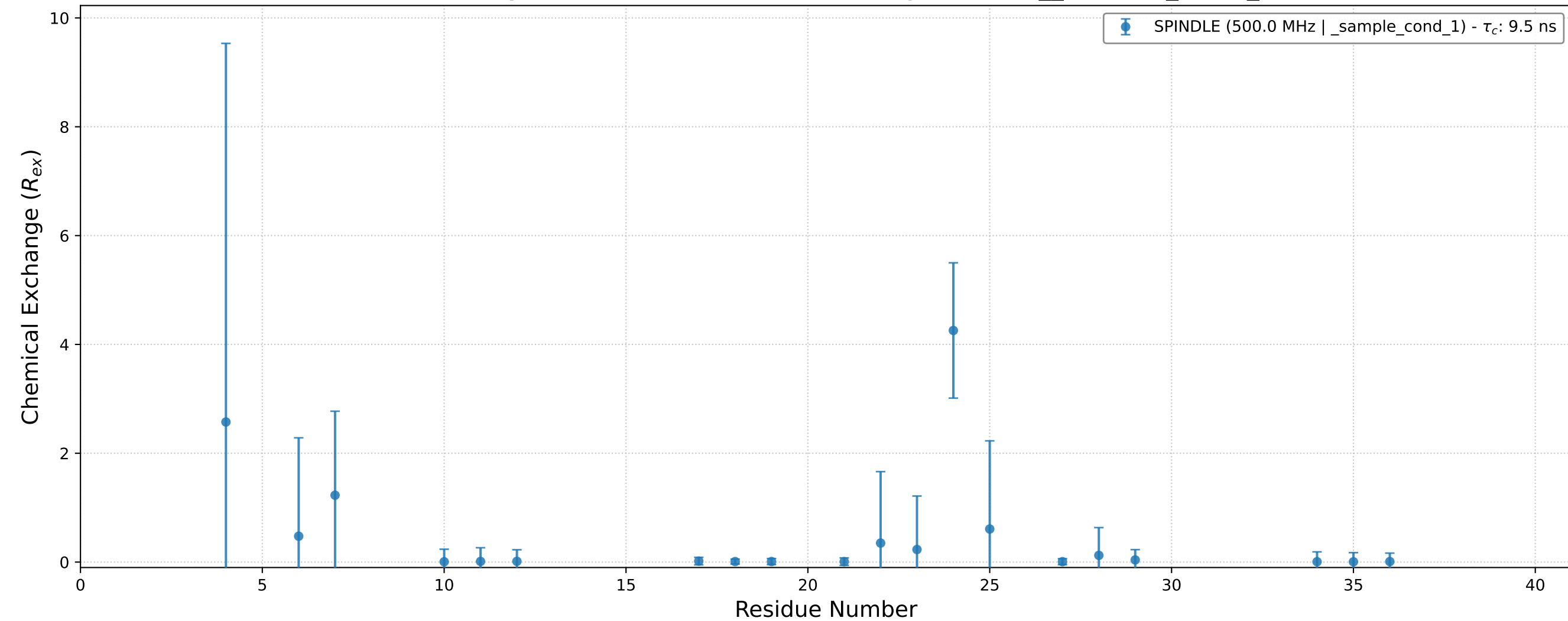
Protein Dynamics Profile ( R_{ex} ) for Target: 5549_sample_cond_1
