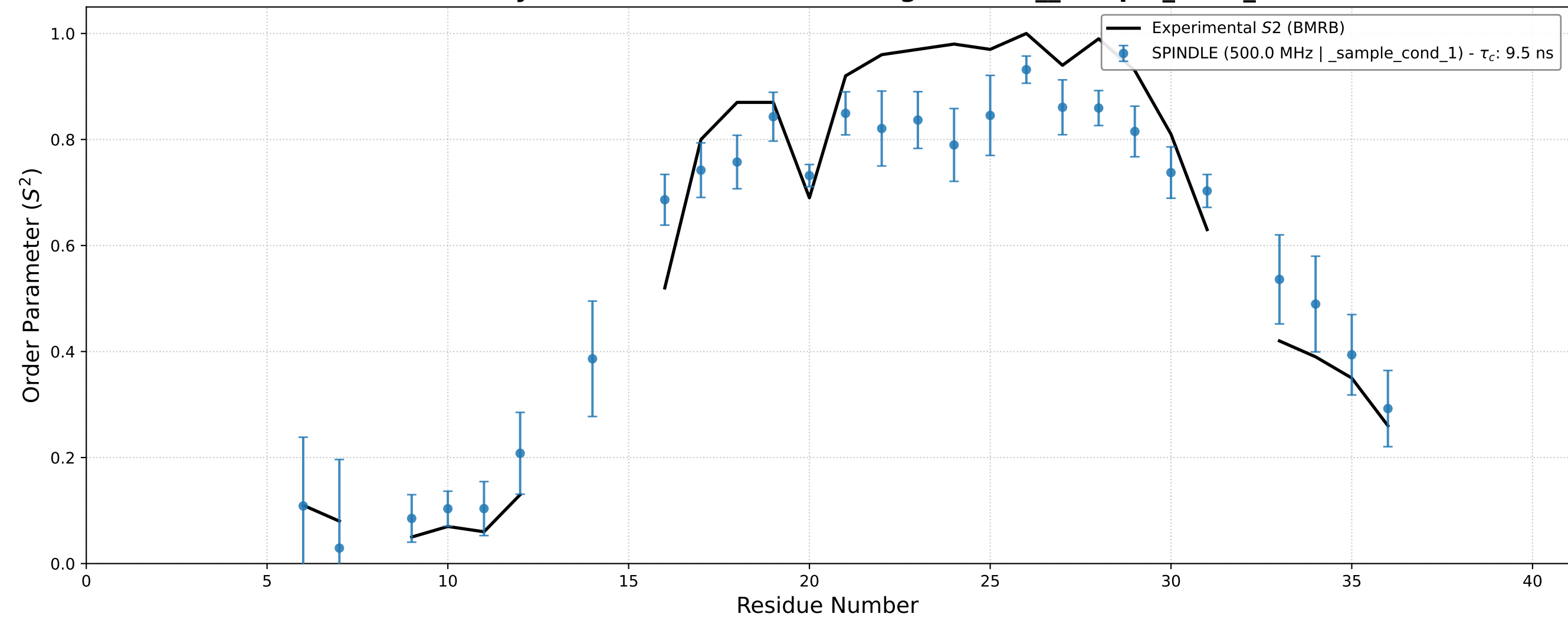
Protein Dynamics Profile ( S^2 ) for Target: 5549_sample_cond_1
