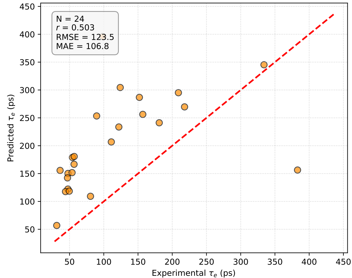
Internal Motion Timescales ( \tau_e )
