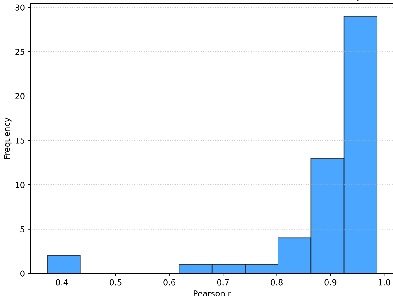
Distribution of S 2 Pearson r Across All Entries (Consensus Only)
