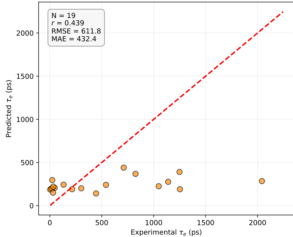
Internal Motion Timescales ( \tau_e )
